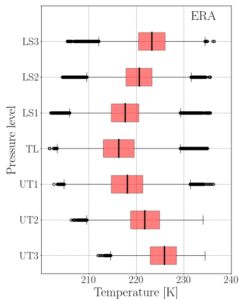
Figure 2. Vertical profile of temperature (K) for IAGOS (blue) and ERA (red).
