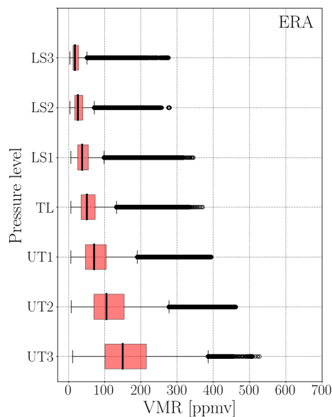
Figure 3. Vertical profile of H 2 O volume mixing ratio (ppmv) for IAGOS (blue) and ERA (red).
