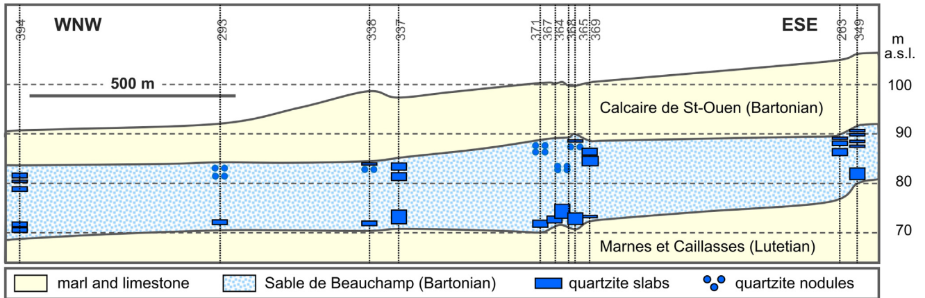
Fig. 8. Selected drillholes along a section through the Sable de Beauchamp formation at Charles de Gaulle airport in Roissy-en-France (Val-d’Oise). The thickness of the silicified layers (especially the thinner layers) has been exaggerated. See position on general geomorphological section in Figure 2 . Drillhole numbers must have the prefix 01545 × 0 to match the national geological data bank (BSS-BRGM – InfoTerre, 2023 ).
