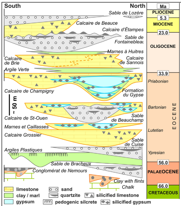
Fig. 3. Schematic diagram of the lithographic succession of the Tertiary deposits in the Paris Basin. Note the wide distribution of the silicified facies within clastic, limestone and gypsum formations (after Thiry, 1999).
