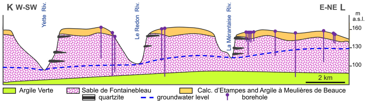
Fig. 6. Section through the incised NW Beauce Plateau (Trappes area). Quartzite pans are limited in distribution to outcrops of the Sable de Fontainebleau. The size of the quartzite lenses is exaggerated for better legibility of the drawing. After Thiry et al. (1988b) .
