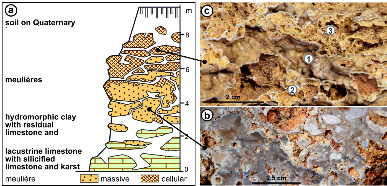
Fig. 21. Weathering features within the Argile à Meulières profile. (a) Macromorphological organisation of the Argile à Meulières profiles. The meulières develop from the silicified limestone by dissolution of the residual limestone domains to form the highly porous ‘cellular’ facies. Modified from Thiry (1999) . (b) Lower massive meulière with secondary silica coating (vitreous-waxy quartzose lustre) on a fracture through micronodules of silicified limestone parent; Bouchy-St-Genest (Marne). (c) Upper cellular meulière facies showing: (1) primary concretionary silica lining voids of silicified limestone to form (2) thin contoured walls, and (3) porous and powdery infilling of hollows resulting from the dissolution of discontinuously silicified limestone matrix; Brie Plateau, St-Cyr-sur-Morin (Seine-et-Marne).
