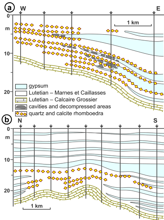
Fig. 13. Quartz pseudomorphs and calcite rhombohedral aggregates in the Late Lutetian Marnes et Caillasses Formation. (a) Seine syncline at Sevran (Seine-Saint-Denis), (b) synclinal trough at Massy (Essonne). After Toulemont (1982).
