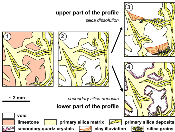
Fig. 22. Schematic showing development of the meulière facies. Dissolution of residual limestone patches (1) generated at first a cellular facies (2). There are two subsequent evolution paths. In the upper part of the profile (3), the silica framework inherited from the silicified limestone was progressively dissolved, voids enlarged, and illuviated clay infiltrated some hollows. In the lower part of the profile (4), secondary euhedral quartz was precipitated in the voids. Adapted from Thiry (1999).
