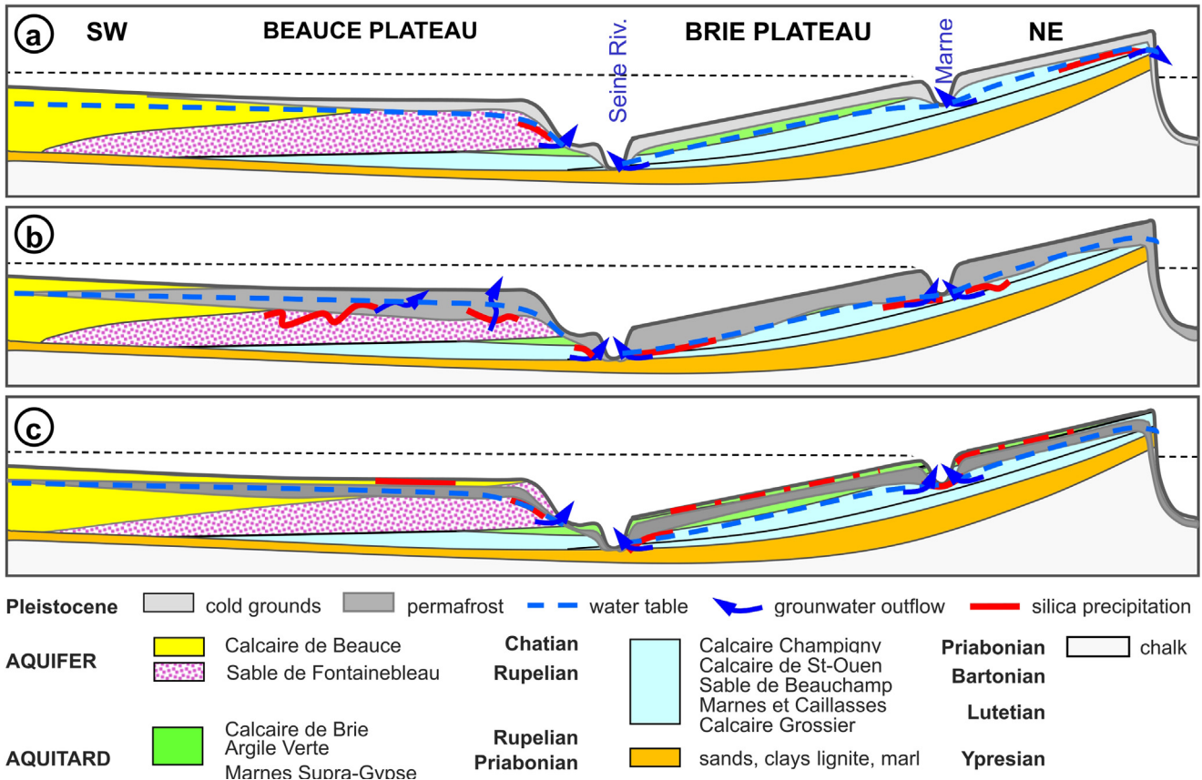
Fig. 25. Conceptual model of hydrological and thermal arrangements within Paris Basin plateaux during Pleistocene glacial periods. (a) At the beginning of the cold period the chilled grounds remained relatively thin and approached the water table level only in its shallowest areas, near springs. (b) With the cold period ongoing, permafrost developed, and the upper parts of the aquifers froze, resulting in overpressures causing ‘forced’ flows along the undulating base of the permafrost and through cracks and taliks. (c) With climate warming the permafrost thawed at its base and at its top. The active layer thickened. A superficial groundwater formed above the permafrost and flowed towards the lowland area. Note that the gradient of the water table and thickness of the permafrost appear reduced on plateau edges due to an extended vertical scale vs horizontal scale.
