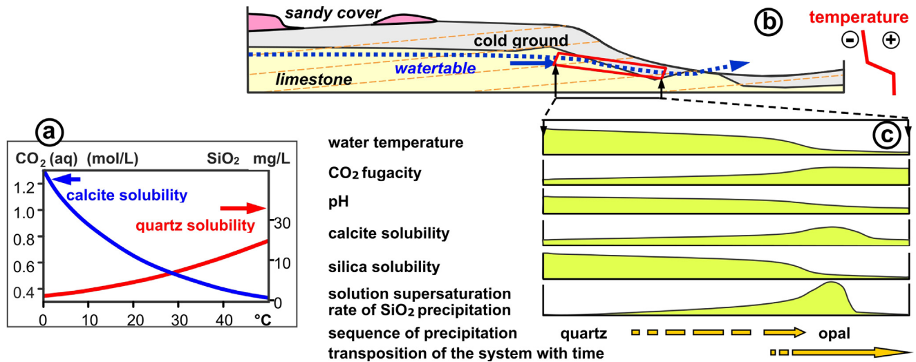
Fig. 20. Geochemical model of limestone silicification during glacial periods. (a) Opposite solubilities of quartz and calcite in water in relation to temperature. (b) Conceptual model of hydrological and thermal arrangements. (c) The interface between cold subsurface and warmer groundwater triggers both precipitation of silica and concomitant microkarstic dissolution of the matrix in the host limestone. Several self-organizing processes explain numerous field and petrographic characteristics of the chert layers.
