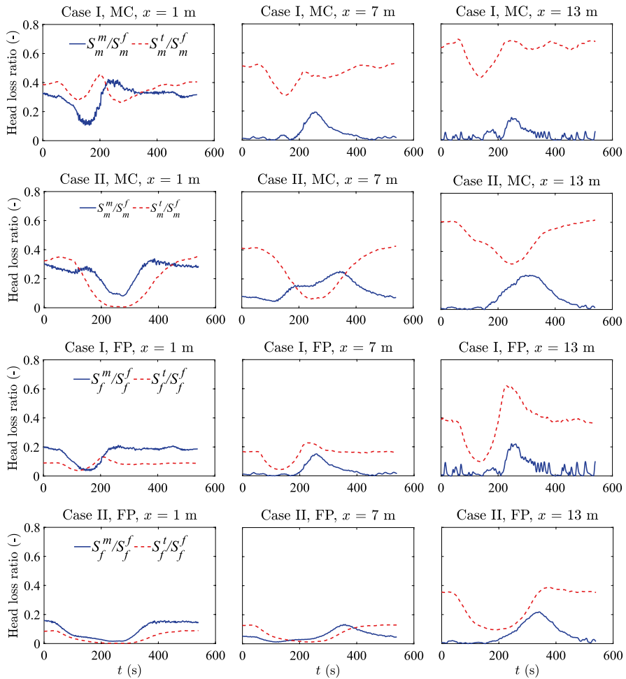
Fig. 11 The three contributions to head losses in MC and FP (see Eqs. 21–22), expressed as the ratio of the head losses by turbulent exchange to the bed-friction slope S_t^t/S_f^f (dashed pink line ‘- - -’), and the ratio of the head losses by depth-averaged lateral mean flow exchange to the bed-friction slope S_m^m/S_m^f (continuous blue line ‘—’), where i = m or f in MC and FP, respectively
