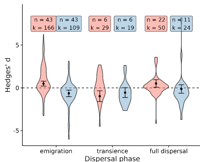
Figure 3: The effect of interactors on focal species dispersal varies depending on the dispersal phase considered
