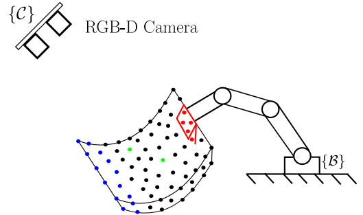
Fig. 1: System configuration. The points depicted on the object are nodes of the volumetric mesh of the 3D object. The red points are nodes attached to the gripper, the green points are the feature points, the blue points are static or free to move, depending on the chosen configuration, and the black points are the other points.
