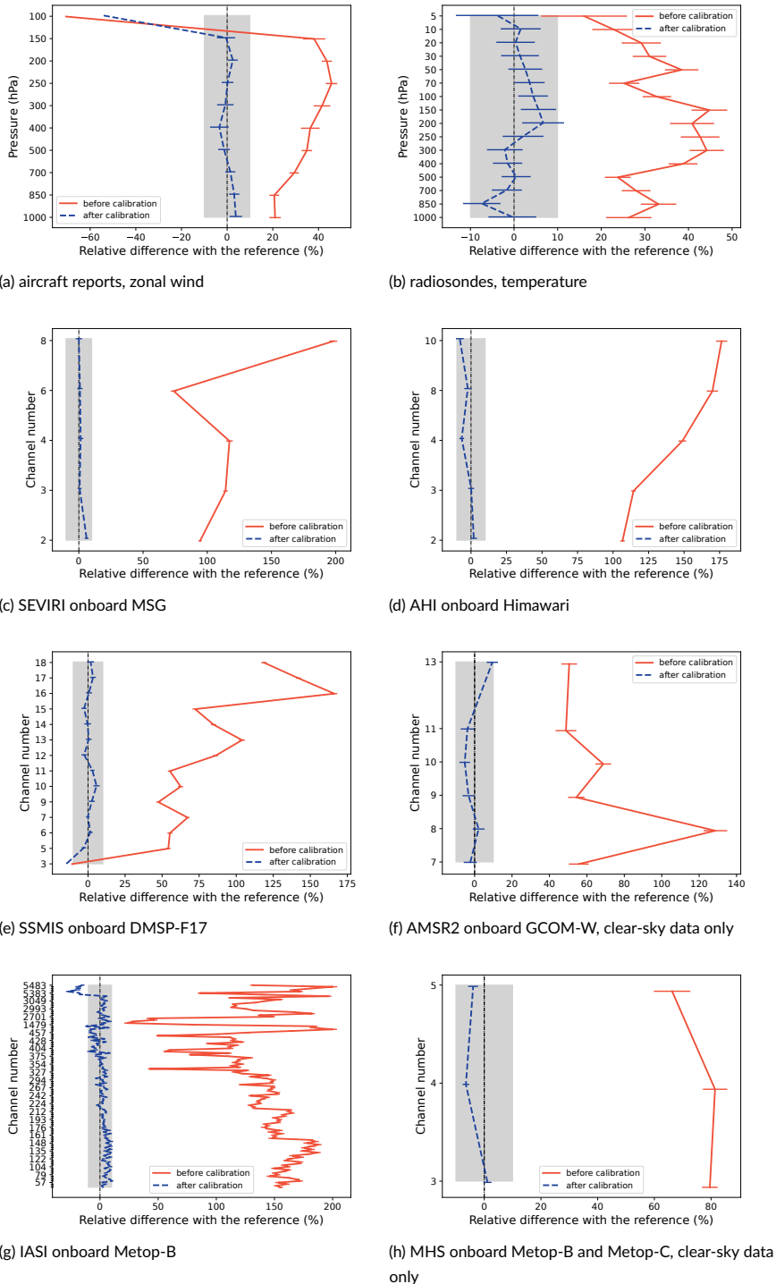
FIGURE 2 Relative first-guess departure standard deviations computed over the globe during 18 days from 14/08/2021 to 31/08/2021, for various observing systems after quality control. The zero line corresponds to first-guess departure standard deviation of real observations. Error bars indicate statistical significant results at the 99% confidence level; in the grey shaded areas, points are at a distance from the reference lower than 10%.
