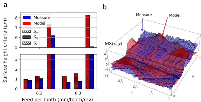
Fig. 7. (a) surface roughness criteria graph comparison between experimental data and the model; (b) machined surface topography (in \mu\text{m} ) comparison between experiment No. 1 and the model
