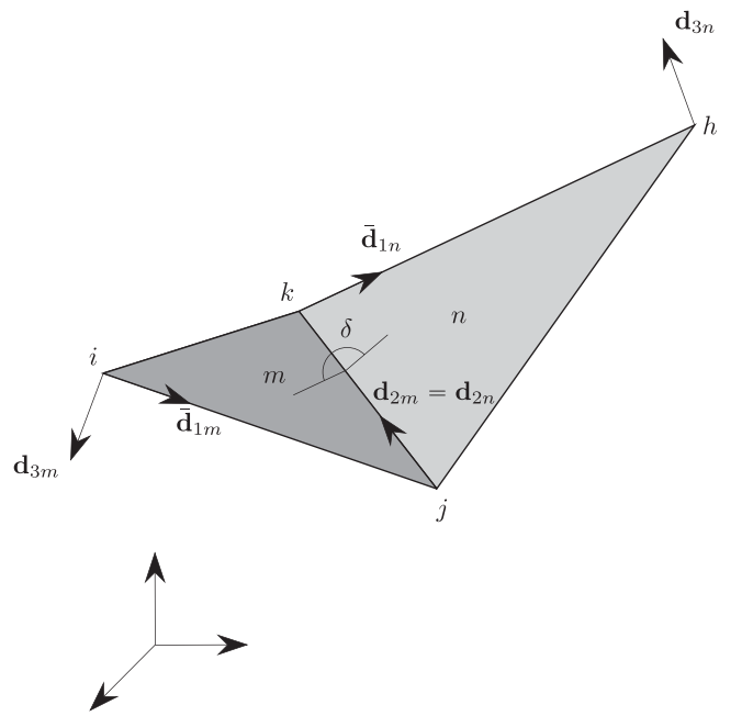
Fig. 3. Deformed configuration of a panel: nodes ( i , j , k and h ), facets ( m and n ) and panel along with the unit vectors ( \mathbf{d}_{3m} , \mathbf{d}_{3n} ) to compute the dihedral angle \delta .
