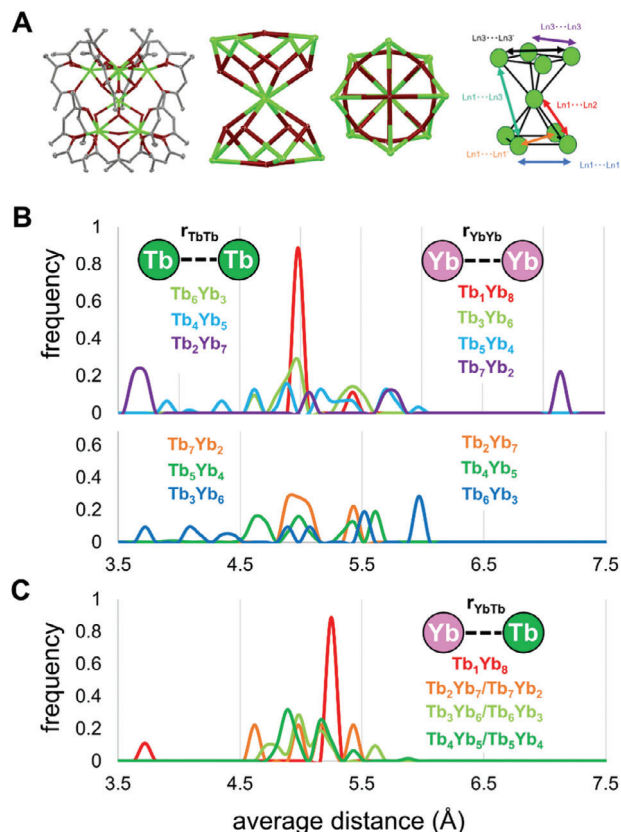
Figure 2. A) Single-crystal X-ray structure of a [Tb_xYb_y(acac)(OH)_9(O)_1] complex ( x = 4.5 , y = 4.5 ), from left to right: Full structure, nonanuclear Ln_9 core, top-down view of Ln_9 core (H-atoms and solvent molecules omitted for clarity, ellipsoids plotted at the 50% probability level), schematic depiction of the nonanuclear core including atom numbering for specific interion distances (CCDC no. 2333808). Frequency distribution of the average B) Yb-to-Yb and Tb-to-Tb and C) Yb-to-Tb distances ( r ) calculated for all isomer configurations of a given Tb_iYb_j complex. Tb_8Yb_1 , Tb_9Yb_0 , and Tb_0Yb_9 are not included because at least 2 Yb ions and 1 Tb ion are necessary for CSU.
