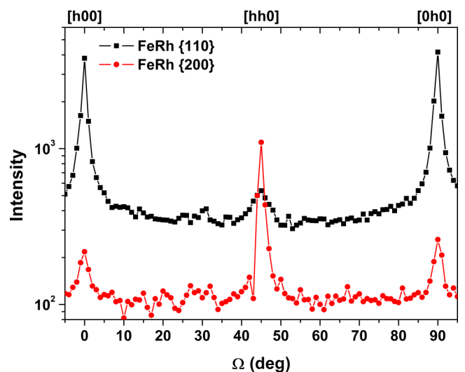
FIG. 6. Intensity of {110} FeRh and {200} FeRh peaks deduced from angular scans, i.e., along different in-plane directions. The background signal coming from the substrate peaks has been subtracted when needed. The higher intensity along particular directions is the signature of preferential orientations (epitaxy relationships).
