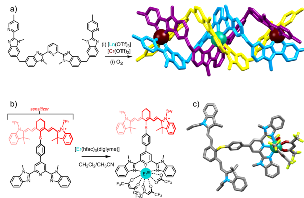
Fig. 6 (a) Heterotrimeric ligand L1 used in the preparation of the heterotrimeric [\text{Cr}_2\text{Er}(\text{L}1)_3]^{9+} complex displaying NIR to visible ETU UC. 29 (b) NIR dye containing tridentate ligand L2 displaying ligand to Er ETU UC. 72 with (c) single-crystal X-ray structure (ion colors: Cr = brown, Er = teal).
