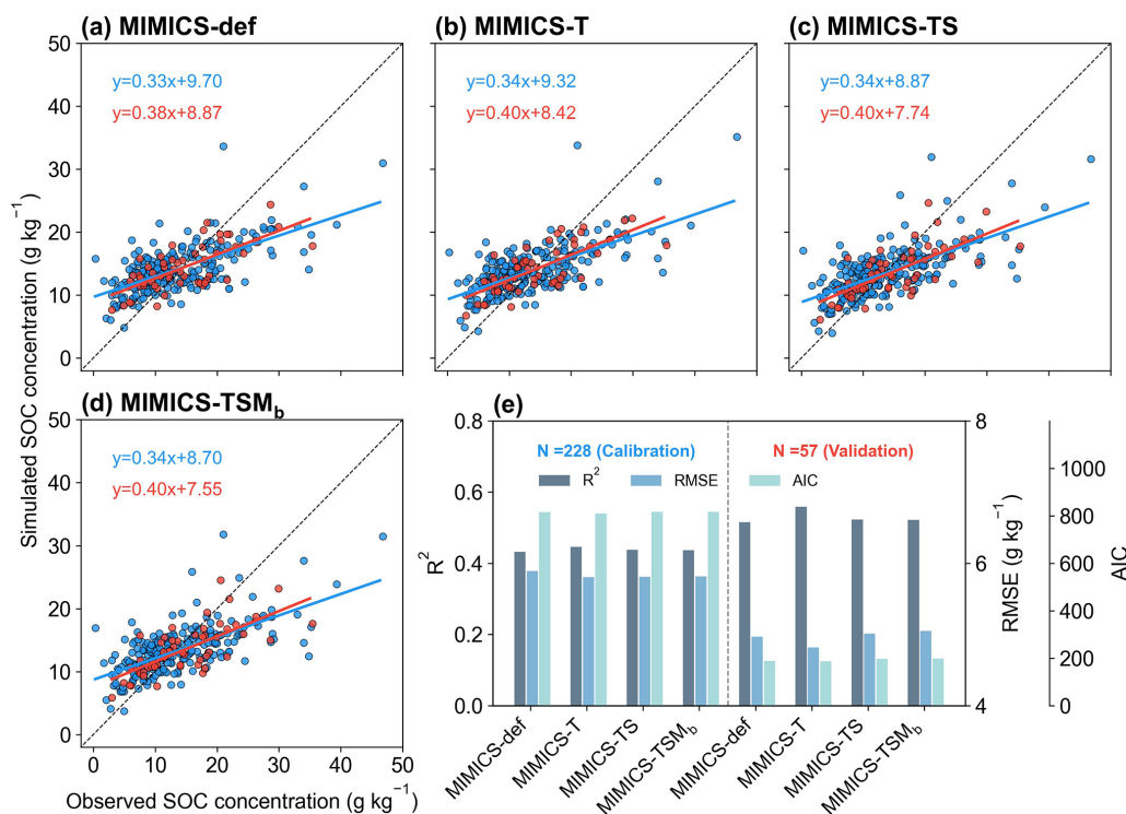
Figure 4. Comparison between the observed and simulated SOC concentrations by (a) MIMICS-def, (b) MIMICS-T, (c) MIMICS-TS, and (d) MIMICS-TSM b . Blue and red dots in panels (a)–(d) represent observation sites for model calibration (80 % sites) and validation (20 % sites), respectively. Panel (e) presents the R^2 , root-mean-square error (RMSE), and Akaike information criterion (AIC) from the model calibration (left) and validation (right) for the four MIMICS versions. The values for the bar graphs in Fig. 4e can be found in Fig. S5. Relationships for the other MIMICS versions can be found in Fig. S9.
