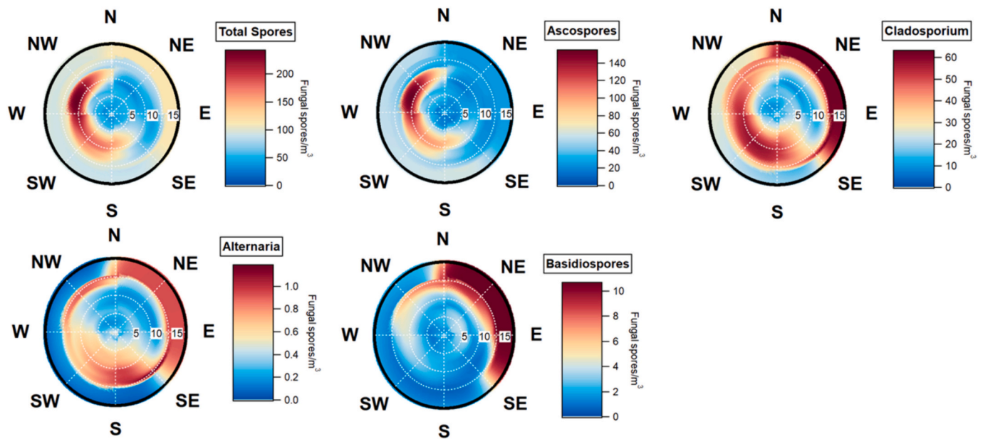
Fig. 4. Origin of Total fungal spores, Ascospores and Cladosporium, Alternaria and Basidiospores spores at sampling site. The colour scale represents the estimated concentration (Spores/m 3 ) white gridlines represent a wind speed scale in kilometer per hour (5 km/h, 10 km/h, 15 km/h, 20 km/h).
