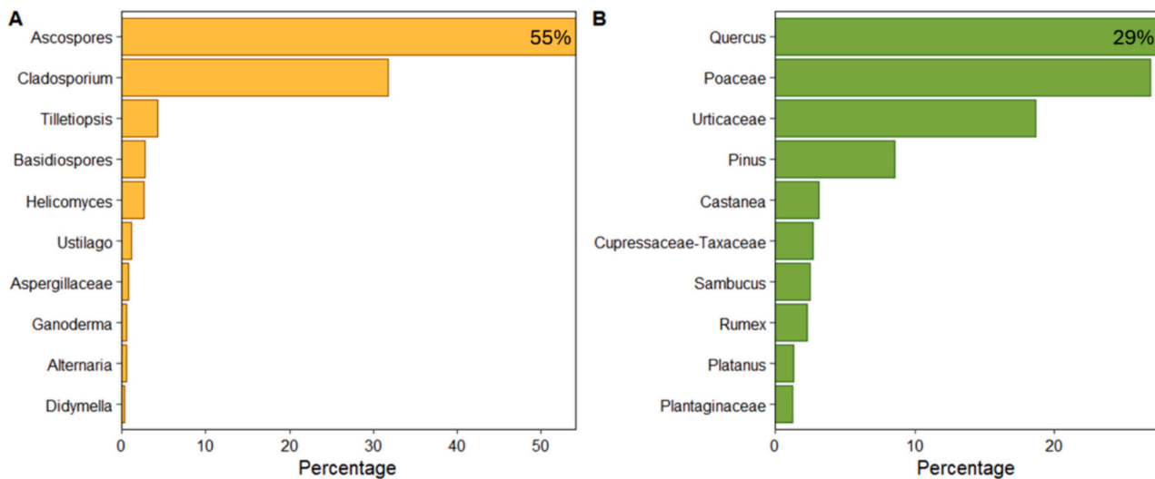
Fig. 1. Percentage distribution of top 10 (A) fungal spore and (B) pollen types.
