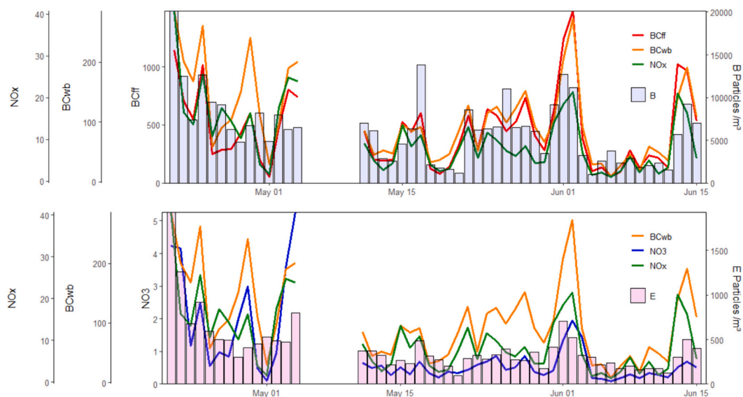
Fig. 5. Comparison between pollutants and (A) B WIBS particles and (B) E WIBS particles.
