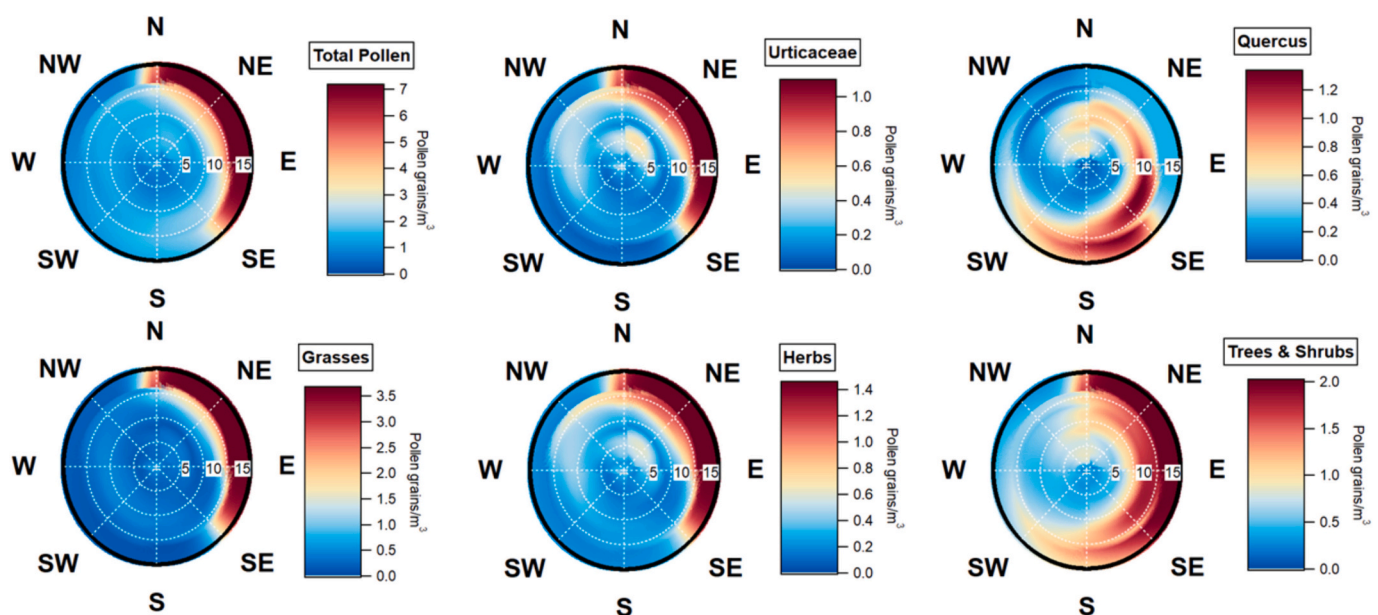
Fig. 3. Origin of Total pollen, Urticaceae, Quercus, Grass, Herb and Tree pollen as sampling site. The colour scale represents the estimated concentration (Pollen grains/m 3 ) white gridlines represent a wind speed scale in kilometer per hour (5 km/h, 10 km/h, 15 km/h, 20 km/h).
