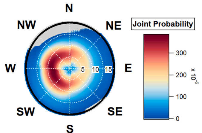
Fig. 2. Wind rose of prevailing winds during sampling period. White broken circles represent a wind speed scale in kilometer per hour (5 km/h, 10 km/h, 15 km/h).
