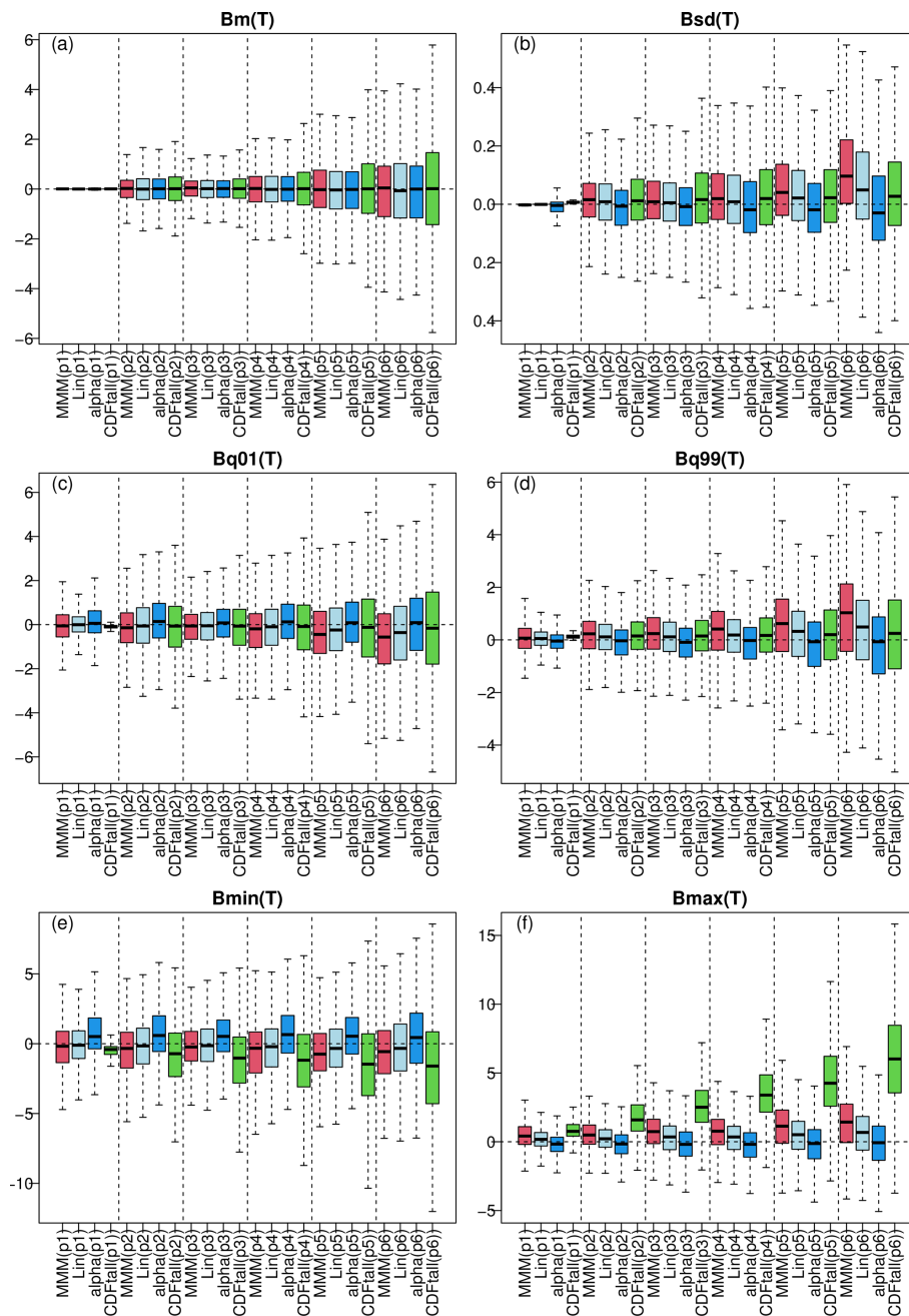
Figure 7. Results of the perfect model experiment for winter temperature: box plots of biases from the three methods (red: MMM, light blue: linear pooling, blue: \alpha pooling, green: CDF-t) for the six 20-year time periods (from p1 for 1981–2000 calibration to p6 for 2081–2100). The different panels display biases in (a) mean temperature, (b) standard deviation, (c) 1 % quantile, (d) 99 % quantile, and (e) minimum and (f) maximum temperature. Note that, for CDF-t, the box plots are drawn from the concatenation of all the individual CDF-t biases. Results for summer are provided in Fig. S9.
