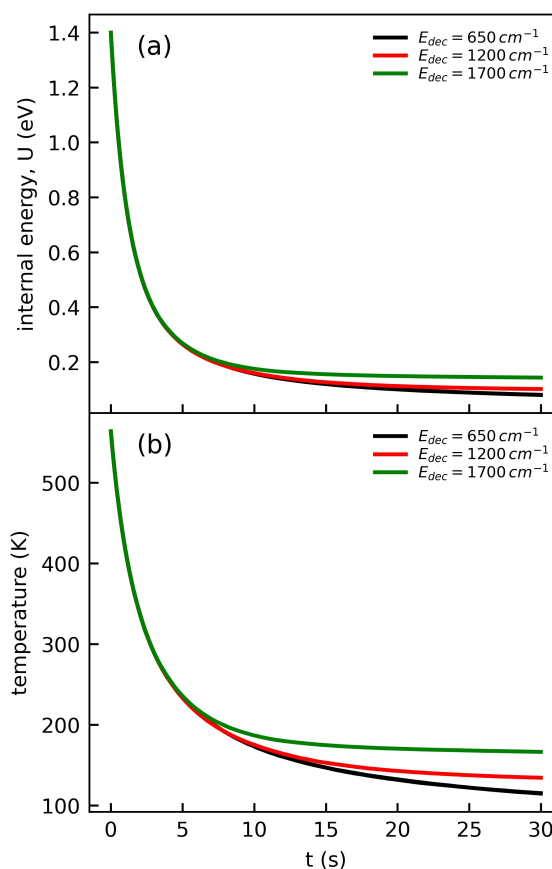
Fig. 14 Time evolution of (a) the internal energy U and (b) the corresponding microcanonical temperature of (N_p)_2^+ computed from the Monte-Carlo model for an initial internal energy U(0) = 1.4 eV and different values of the decoupling energy, E_{dec} .
