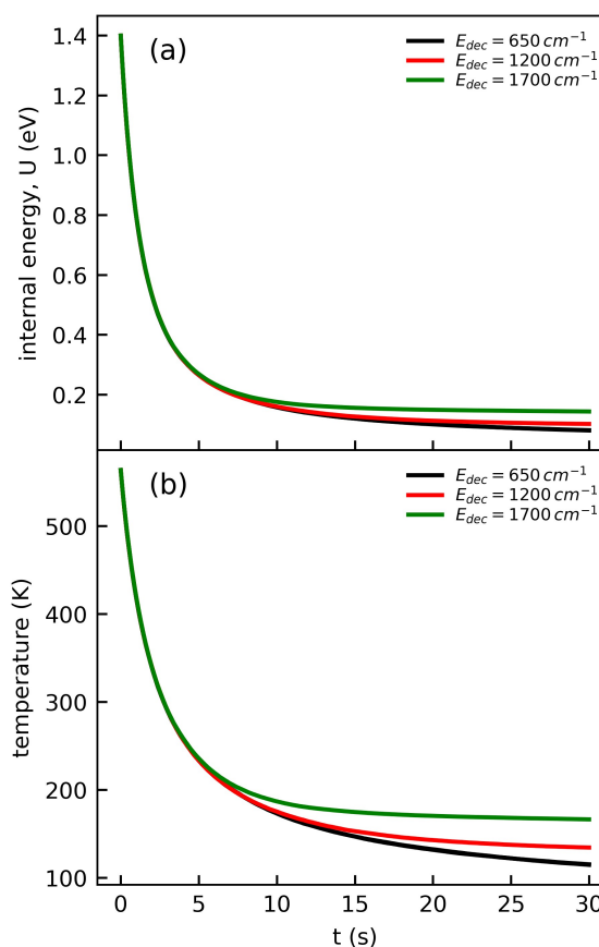
Fig. 14 Time evolution of (a) the internal energy U and (b) the corresponding microcanonical temperature of (Np)_2^+ computed from the Monte-Carlo model for an initial internal energy U(0) = 1.4\text{ eV} and different values of the decoupling energy, E_{dec} .
