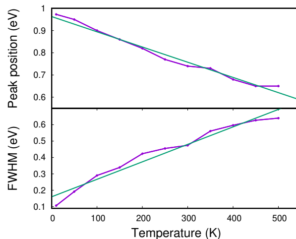
Fig. 13 Theoretical energy position of the maximum (upper panel) and width (lower panel) of the CR band as functions of temperature. The green lines are linear fits to the calculated data (see text).
