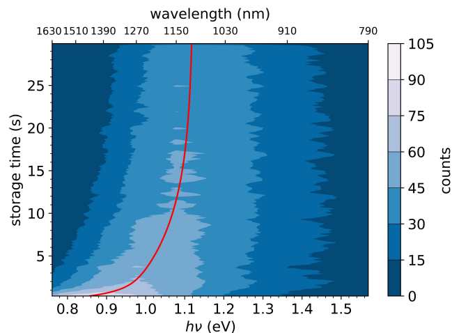
Fig. 6 Action spectra of laser-induced naphthalene-dimer dissociation, (C_{10}H_8)_2^+ \rightarrow C_{10}H_8^+ + C_{10}H_8 . The intensity, as a function of the storage time before the firing of the laser and the laser photon energy, is shown through the color scale shown to the right. The red line is an exponential fit of the CR band position determined at maximum intensity, showing the shift of the CR band position with storage time.
