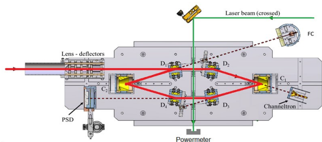
Fig. 5 Schematic of the room-temperature Mini-Ring in Lyon. Red arrows show the main path of the stored (C_{10}H_8)_2^+ dimer cations. The green arrow symbolizes the perpendicular crossing of the laser beam with the stored ions. Note that due to well-controlled time matching between the ions bunch and the laser nanosecond pulses, the crossing only occurs between defectors D_3 and D_4 . The neutral fragments resulting from prompt laser dissociation are detected by the position-sensitive detector, PSD.
