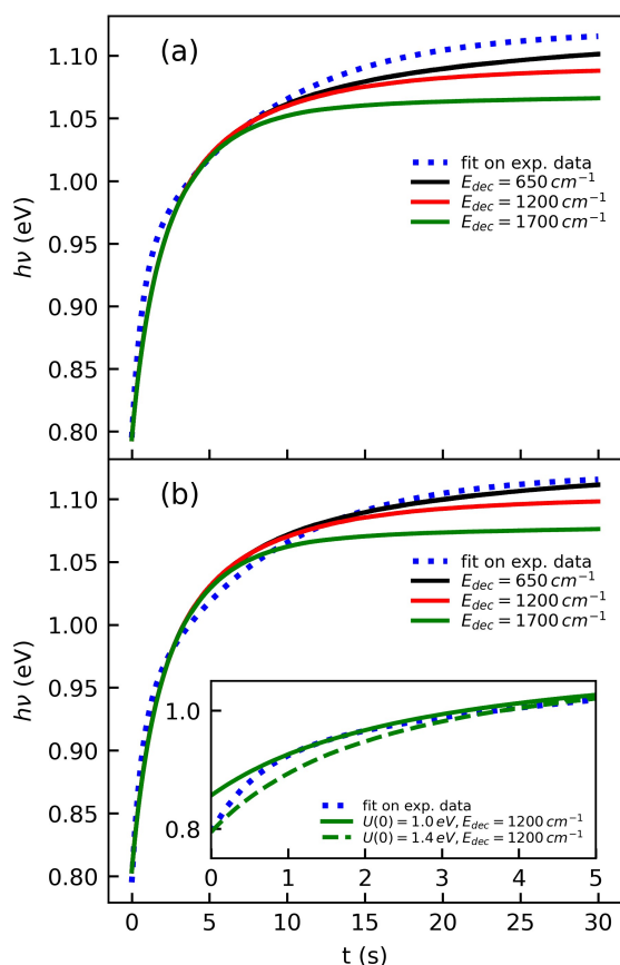
Fig. 15 Simulations of the time evolution of the CR band position of (\text{Np})_2^+ and comparison with the fitted experimental curve (Eq. 1). The simulated curves were obtained by combining the results from a kinetic Monte Carlo radiative cooling model with the temperature dependence of the position of the CR band using Eq. 7. The parameters in the model are U(0) , the initial internal energy, E_{dec} , the decoupling energy, and the reference position h\nu_0 in Eq. 7. The simulated curves shown correspond to (a): U(0) = 1.4 eV, h\nu_0 = 1.18 eV for different values of E_{dec} . (b): similar to case (a) but with U(0) = 1.0 eV and h\nu_0 = 1.19 eV. The inset illustrates the effect of U(0) in the short time range.
