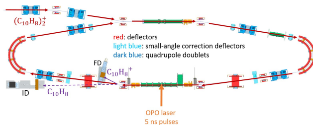
Fig. 2 Schematic of the cryogenic asymmetric ring of DESIREE. Red arrows show the main path of the parent (C_{10}H_8)_2^+ dimer cations stored in DESIREE. The orange arrow symbolizes the perpendicular crossing of the laser beam with the stored ions. The neutral and charged fragments resulting from laser dissociation are detected by the imaging detector (ID) and the fragment detector (FD), respectively. Spontaneous dissociation of internally hot (C_{10}H_8)_2^+ dimer cations occurring in this straight section also contributes to events recorded by those detectors.
