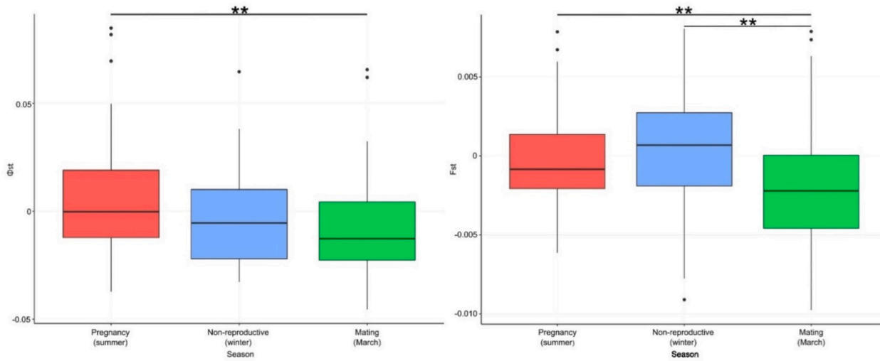
Fig. 3. Temporal differences in \Phi_{st} (mtDNA) and F_{st} (microsatellites) values between seasons in Mormopterus francoismoutoui . ** p < 0.01 (Tukey's post-hoc tests).
