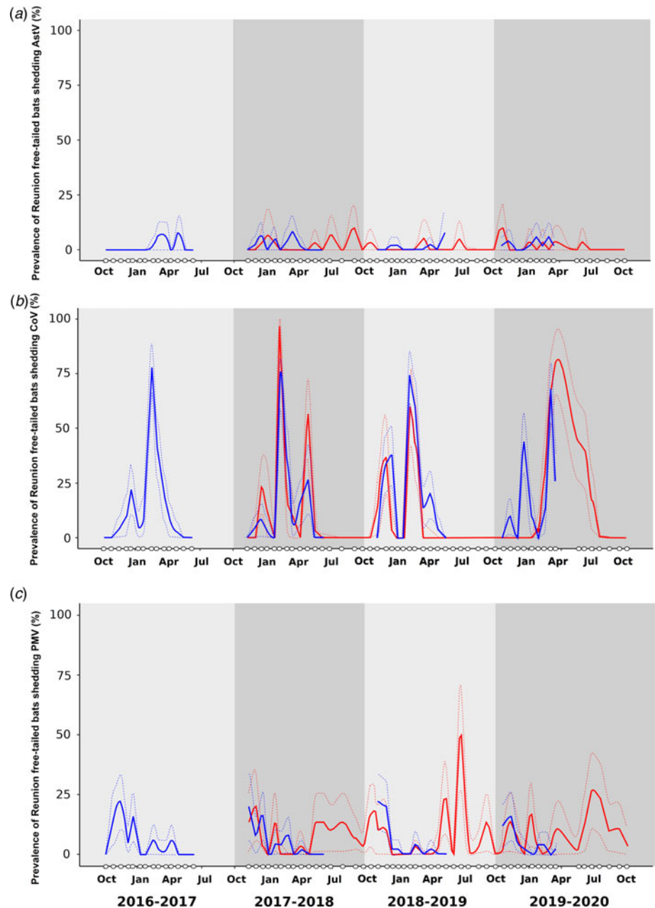
Fig. 1. Prevalence of Reunion free-tailed bat ( Mormopterus francoismoutou ) shedding astrovirus (AstV; a), coronavirus (CoV; b) and paramyxovirus (PMV; c), during four consecutive seasons (October 2016 to October 2020). White dots on x-axis indicate sampling dates. Continuous lines represent the proportion of positive samples and were predicted with a loess function in R. Dashed lines represent the 95% confidence interval. Blue: cave (occupied by bats from October to May); red: building (occupied all year long).
