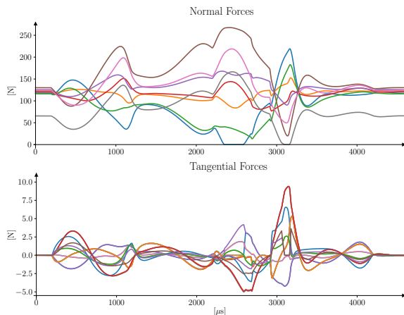
Fig. 7: Contact forces.
