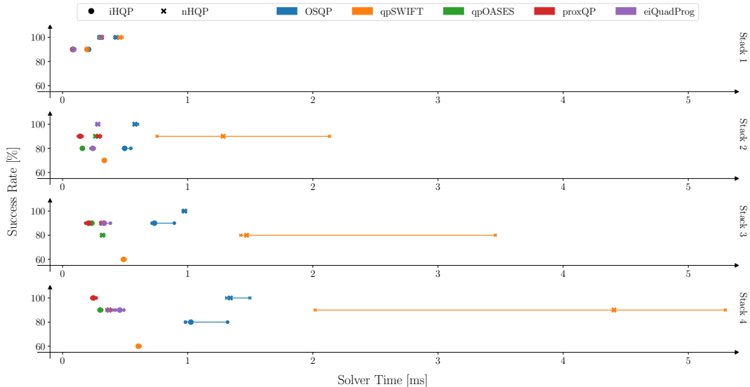
Fig. 3: 29 DOFs humanoid robot benchmark.
