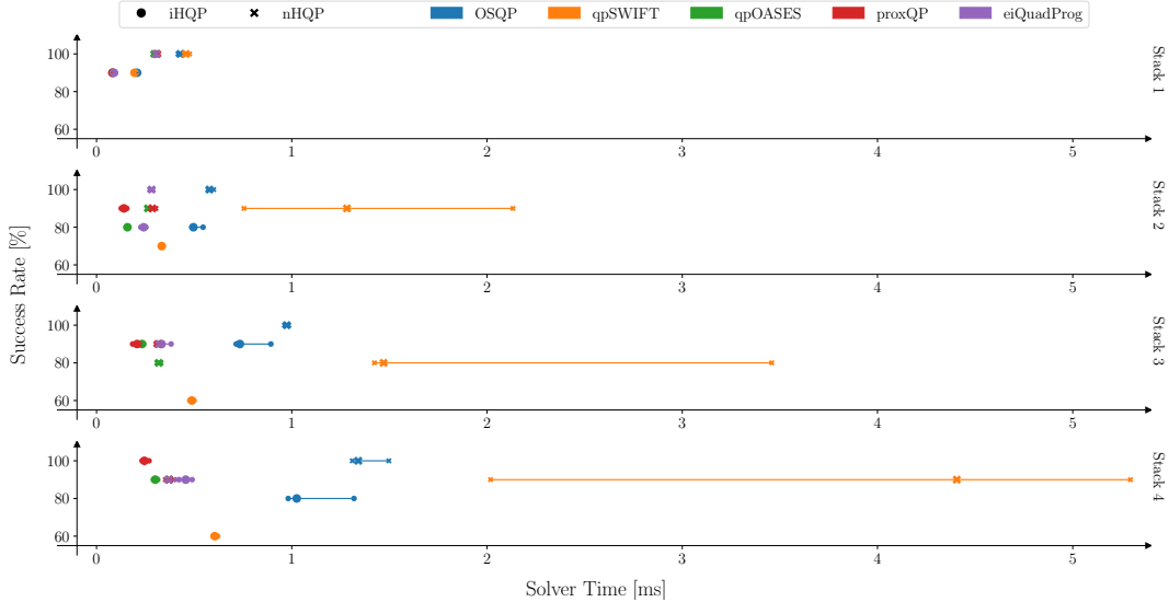
Fig. 3: 29 DOFs humanoid robot benchmark.
