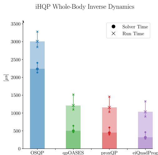
Fig. 5: Comparison between different back-ends running the whole-body inverse dynamics on the TALOS robot using the iHQP front-end. The run time considers the solver time, the update of the model and the stack, and a small overhead due to the communication to ROS provided by the CartesI/O framework.
