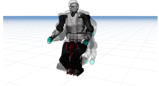
Fig. 4: Open loop whole-body inverse dynamics performed on TALOS model.
