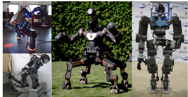
Fig. 1: Some of the robots that utilized OpenSoT as a whole-body motion engine include MARM in the top-left, COMAN+ in the bottom-left, CENTAURO in the center, and WALK-MAN on the right.
