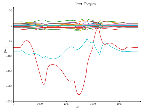
Fig. 6: Computed torques.
