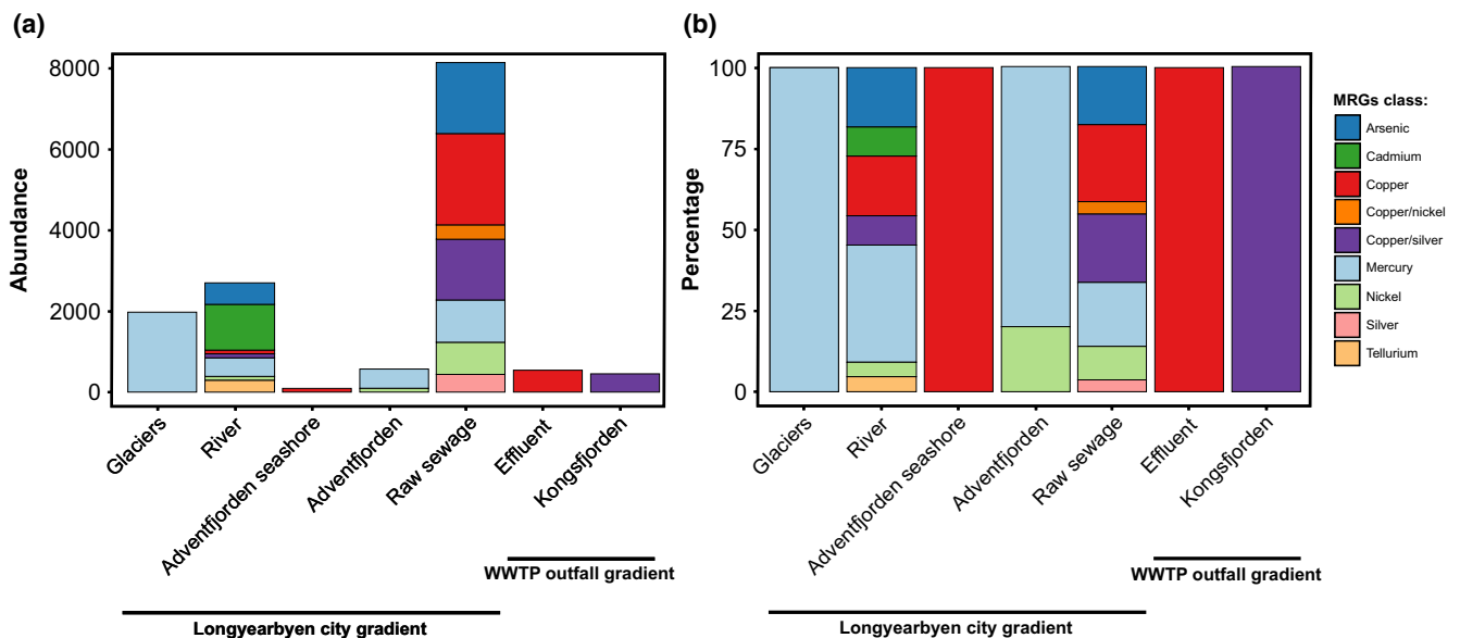
FIGURE 5 (a) Abundance and (b) percentage of MRG classes detected across the plasmidome from environments with different anthropogenic pressures: glacial environment, marine environment, WWTP, and receiving water. MRG, metal resistance gene; WWTP, wastewater treatment plant.
