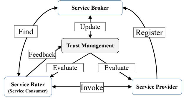
Fig. 2: SOA-based TM
