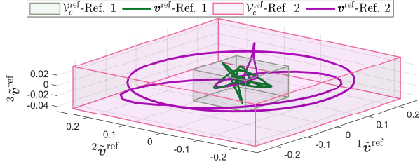
Fig. 3. Two input v^{\text{ref}} of the two references and their bounding boxes.
