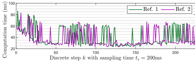
Fig. 7. Computation time for the proposed MPC scheme.
