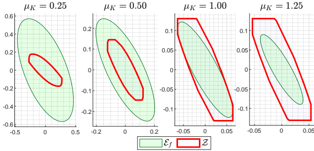
Fig. 4. Effect of changing the gain K towards fast closed-loop convergence, projected into the first two axes of \tilde{x}_k ( ^1\tilde{x}_k -horizontal, ^2\tilde{x}_k -vertical).
