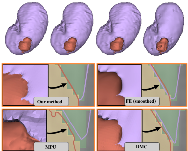
Fig. 12. Reconstruction of a kidney with a tumor from the 2019 KiTS Challenge [55, 56]: on top, the built 3D models, from left to right: our method, FE(smoothed), DMC, MPU. By using MPU or DMC, an empty space between the surface of the reconstructed kidney and tumor is exhibited, while with FE, overlaps appear due to surface smoothing (FE, DMC and MPU do not use any topological solution).
