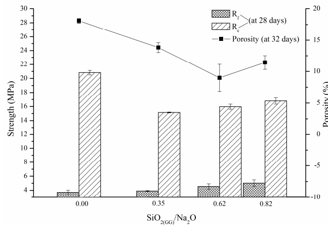
FIGURE 6. Mechanical strength and porosity of mortars with different \text{SiO}_2(\text{GG})/\text{Na}_2\text{O} ratio
