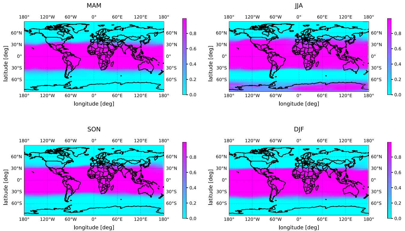
Figure 3. The fraction of Terrestrial Gamma-ray Flashes above detection threshold mapped on the globe, for each season of the year.
