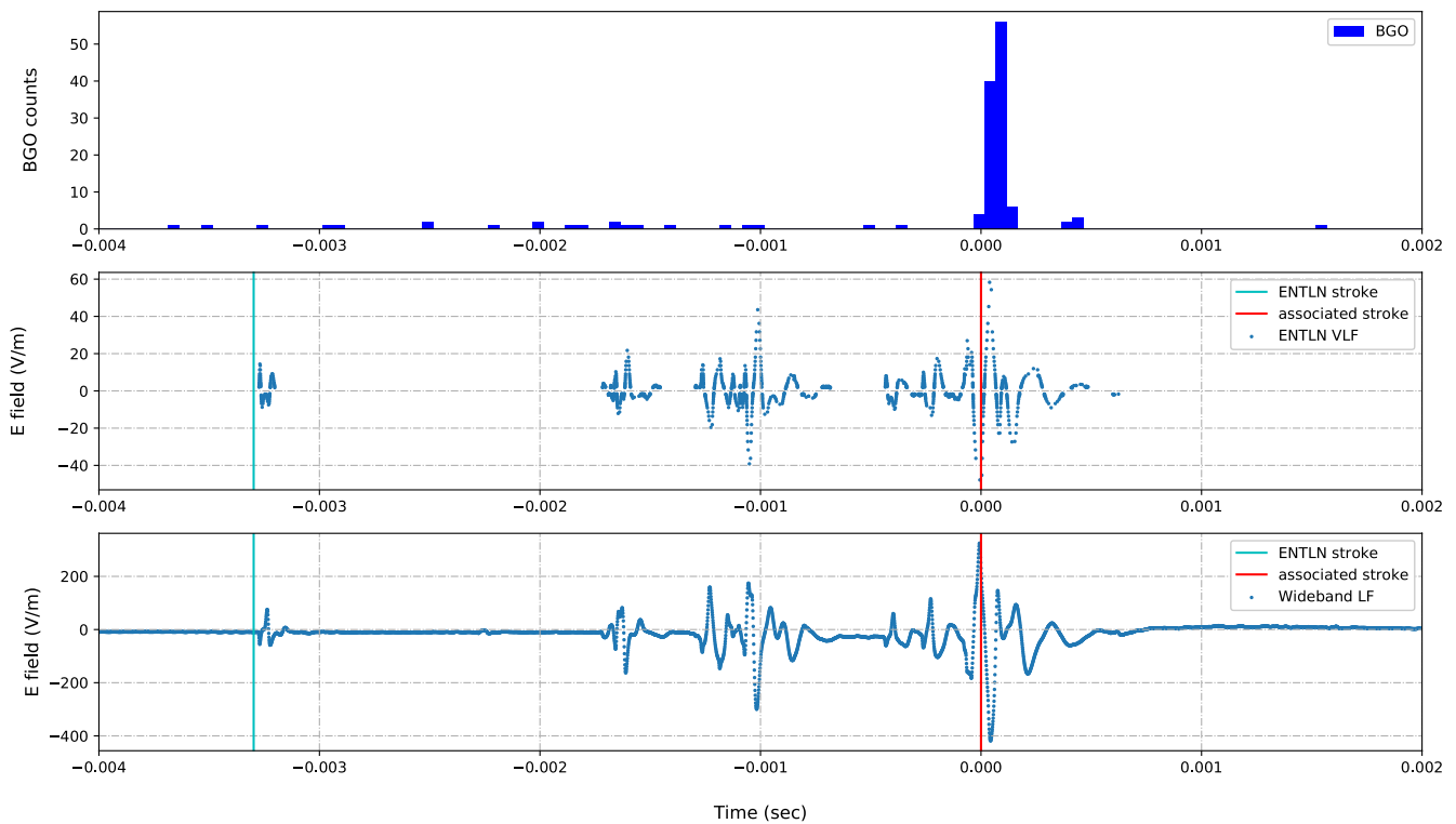
Figure 10. Top: the Bismuth-Germanium Oxide lightcurve, with a bin size of 50 \mu\text{s} . Middle: the radio waveform recorded by Earth Networks Total Lightning Network for the associated stroke. Bottom: the radio waveform as recorded by the authors (Füllekrug). Here the Terrestrial Gamma-ray Flashes is matched to the second sferic based on the largest peak current (see main text).
