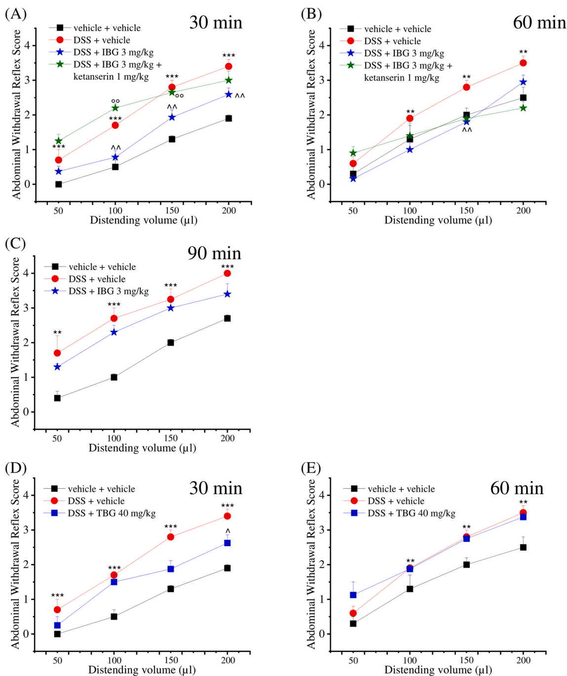
Fig. 4. Effect of the acute administration of IBG and TBG on DSS-induced visceral pain in mice. Animals were treated with DSS (●), or vehicle (■), for 5 consecutive days to induce hyperalgesic pain. On day 8, mice were administered (i.p.) 3 mg/kg IBG (★) (A-C) or 40 mg/kg TBG (■) (D,E), or vehicle (■). Visceral sensitivity was assessed by measuring the extent of the AWR to colorectal distension (50–200 µL) at 30 min (A), 60 min (B), and 90 min (C) for IBG, and at 30 min (D) and 60 min (E) for TBG. To determine the role of the -5\text{-HT}_{2A} receptor, ketanserin (1 mg/kg) was injected (i.p.) 30 min before IBG (3 mg/kg) (★) (A,B). Each value represents the mean \pm SEM of 6–8 animals per group performed in two different experimental sets. Statistical analysis of the results showed that DSS (●) induces visceral pain in the 30–90 min time regime (** p < 0.01 and *** p < 0.001 vs vehicle + vehicle), and that IBG (★) at 30 min ( \Delta p < 0.01 at 100–200 µL) (A) and 60 min ( \Delta p < 0.01 at 150 µL) (B), and TBG (■) at 30 min ( \Delta p < 0.05 at 200 µL) (D) significantly improve visceral pain, compared to DSS + vehicle-treated animals (●). Ketanserin completely counteracted the anti-hypersensitivity effect observed for IBG (★) at 30 min ( \Delta p < 0.01 at 100–150 µL) in comparison to the respective ibogalogue-treated mice.
