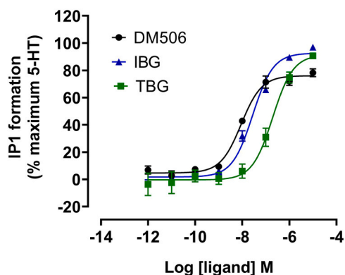
Fig. 5. Functional activity of DM506, IBG, and TBG at the human 5-HT 2A receptor. NIH/3T3 cells expressing this receptor subtype were incubated (90 min) with different concentrations of DM506 (●), IBG (▲), or TBG (■). Activation of the 5-HT 2A receptor was assessed by IP1 formation. Receptor activation data were normalized considering 0% as the baseline signal and 100% as the maximum 5-HT-stimulated signal. Data are shown as mean ± SEM from at least three experiments, each performed in triplicate. The calculated EC 50 and E max values are summarized in Table 3.
