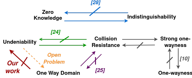
Fig. 1. Relations between security properties of accumulators.
