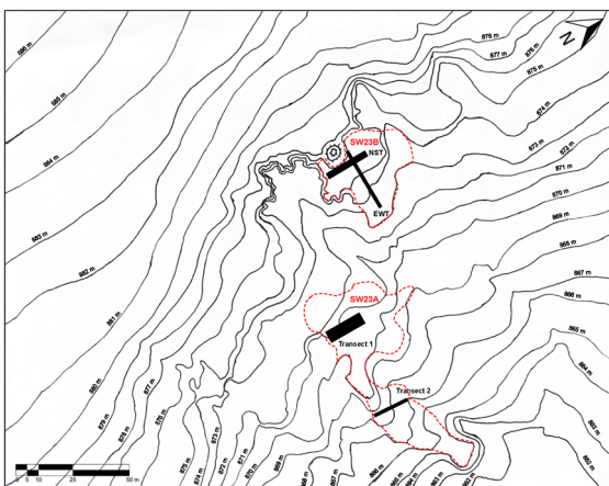
Fig. 3 Contour map showing SW23A and B. The dashed lines indicate the edges of the artifact scatters on each spur, and the black rectangles are the locations of the transects collected in 2019. Contour interval is 1 m
