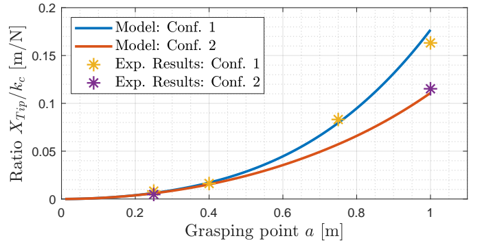
Fig. 11. Ratio X_{Tip}/k_c for different grasping points a . The proposed model (see Equation (32)) is represented in a blue line, while the markers represent the slope of the linear interpolation of the experimental data, represented in Figure 10.
