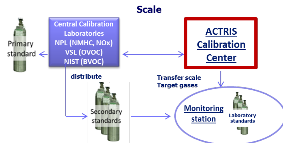
Figure 2: Scheme demonstrating how the SI traceable scale of reactive trace gases should be maintained and transferred to the National Facilities.
