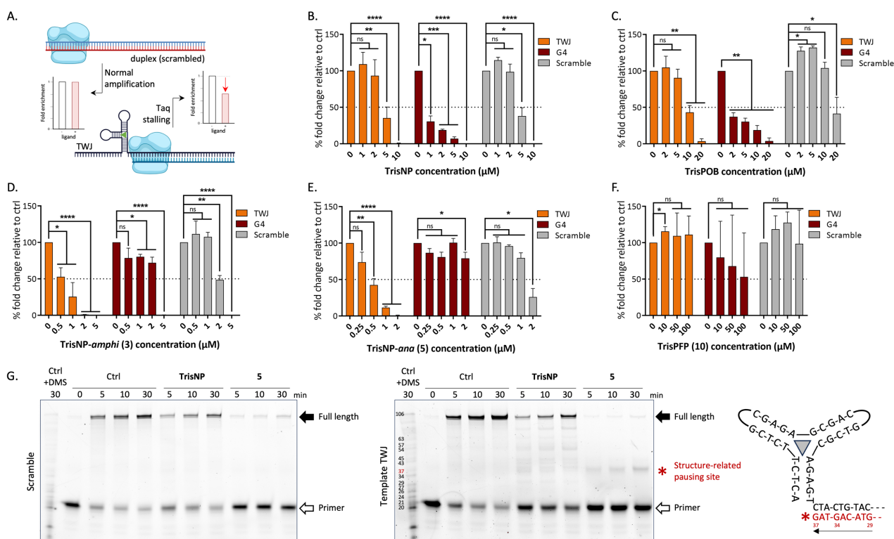
Figure 4. A) Principle of the qPCR stop assay. B-F) Evaluation of the ability of TrisNP (B), TrisPOB (C) (as references) and three out of five most promising candidates (D: compound 3 ; E: compound 5 ; F: compound 10 ; results for compounds 9 and 11 in Figure S1) to inhibit in vitro polymerization by the qPCR Stop assay, quantified as relative amplification (% fold change) of structured (TWJ or G4) or control (Scramble) templates (2 pM). Data are means \pm s.d. from at least 3 independent experiments performed in duplicates; statistical analyses were performed with multiple unpaired t-tests: ns: p > 0.05 ; *: p < 0.05 ; **: p < 0.01 ; ***: p < 0.001 ; ****: p < 0.0001 . G) Taq polymerase stop assays performed with the scramble and TWJ-containing templates (the G4 template in Figure S4) without or with ligands ( TrisNP and 5 ); reactions were performed at 50 °C, stopped after 5, 10 or 30 min and then loaded on a denaturing 12% (v/v) polyacrylamide gel (quantification in Figure S4). Right panel: schematic representation of a ligand-stabilized TWJ that acts as a structural roadblock able to pause polymerization (the pausing site is labelled with a *; loops are T 6 ).
