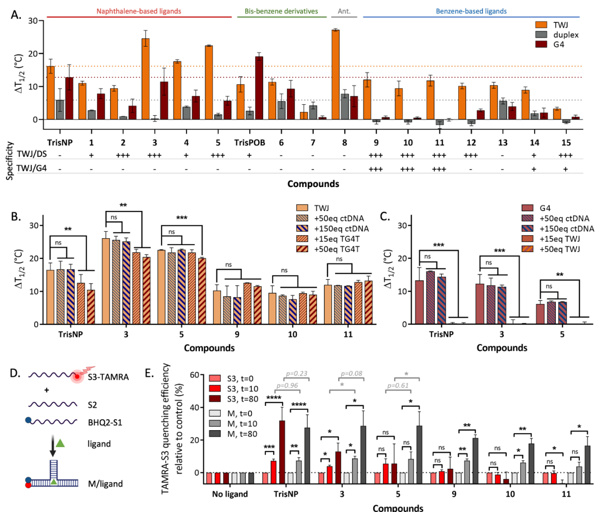
Figure 3. A) Evaluation of the apparent affinity of 17 azacryptands by FRET-melting assays performed with TWJ, DS and G4. Assays were performed with 0.2 \mu\text{M} of each double-labelled DNA structure and 1.0 \mu\text{M} of each ligand in appropriate buffer. The specificity score is estimated on the basis of the \Delta T_{1/2}^{\text{TWJ}}/\Delta T_{1/2}^{\text{G4}} or \Delta T_{1/2}^{\text{TWJ}}/\Delta T_{1/2}^{\text{DS}} ratio (+++: \geq 10 ; +: \geq 4 ) or the lack of DS/G4 stabilization ( \Delta T_{1/2} < 4 ). Dotted lines correspond to TrisNP results. B) Evaluation of the TWJ-selectivity of the five most promising candidates plus TrisNP by competitive FRET-melting experiments performed with FAM-TWJ-TAMRA in the absence or presence of 10 and 30 \mu\text{M} ctDNA, or 3 and 10 \mu\text{M} TG 4 T as competitors. The increase in \Delta T_{1/2} values in the presence of an excess of competitors (e.g., 9 and 11 ) is often observed for highly selective ligands and likely originates in an increase of ionic strength in the experimental medium. C) Evaluation of G4-DNA binding of 3 , 5 and TrisNP by competitive FRET-melting experiments performed with FAM-G4-TAMRA in the absence or presence of 10 and 30 \mu\text{M} ctDNA, or 3 and 10 \mu\text{M} TWJ as competitors. D) Principle of the modified TWJ-Screen assay (blue sphere = BHQ2; red sphere = TAMRA; green triangle = ligand). E) Evaluation of the ability of the five most promising candidates plus TrisNP to promote TWJ formation by the TWJ-Screen assay, quantified by the relative quenching of S3-TAMRA fluorescence when mixed with BHQ2-S1 and S2 (M, 0.2 \mu\text{M} ) and the ligand (1.0 \mu\text{M} , the mixture of S3-TAMRA+ligand being used as a control) as a function of the time. Statistical analyses were performed with multiple unpaired t-tests: ns: p > 0.05 ; *: p < 0.05 ; **: p < 0.01 ; ***: p < 0.001 ; ****: p < 0.0001 .
