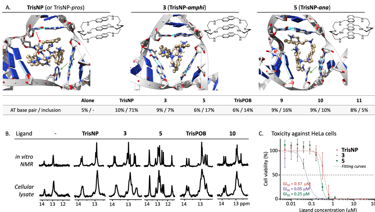
Figure 5. A) Representative conformations of TrisNP , 3 and 5 bound in a TWJ obtained via molecular dynamics (MD, representative structure after clustering one 2- \mu\text{s} -long simulation), along with the quantification ( n = 10 ) of AT base pair and of the inclusion complex persistence as a percentage of the total MD simulation time. The transient inclusion complex in which nucleobases are sandwiched inside TrisNP is indicated with a red arrow, the unpaired nucleobases with green arrows (the structures of the complexes with TrisPOB , 9-11 can be seen in Figure S5). B) Imino regions of ^1\text{H} NMR spectra of 100 \mu\text{M} TWJ before and after the addition of one molar equivalent of ligands ( TrisNP , TrisPOB , 3 , 5 , 10 ). The spectra were acquired at 37 ^\circ\text{C} in vitro (130 mM KCl, 20 mM KPOi, pH 7.2) or in crude homogenate from HeLa cells. C) Antiproliferative activity of TrisNP , 3 and 5 against cervical cancer cells (HeLa) evaluated by the SRB assay ( n \geq 3 ).
