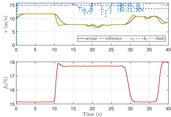
Fig. 15: Quintic speed profiling - sc3.
