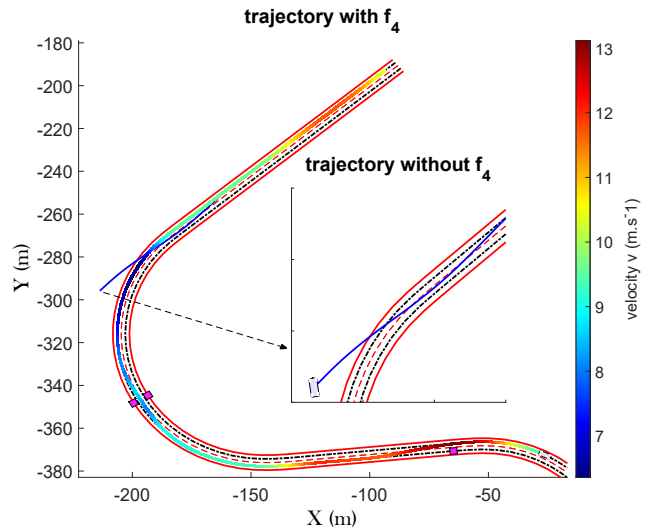
Fig. 14: Vehicle trajectory (same legend as Fig. 2) - sc2.
