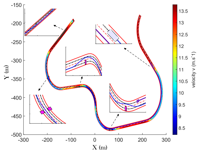
Fig. 9: Vehicle trajectory (same legend as Fig. 2) - sc1.
