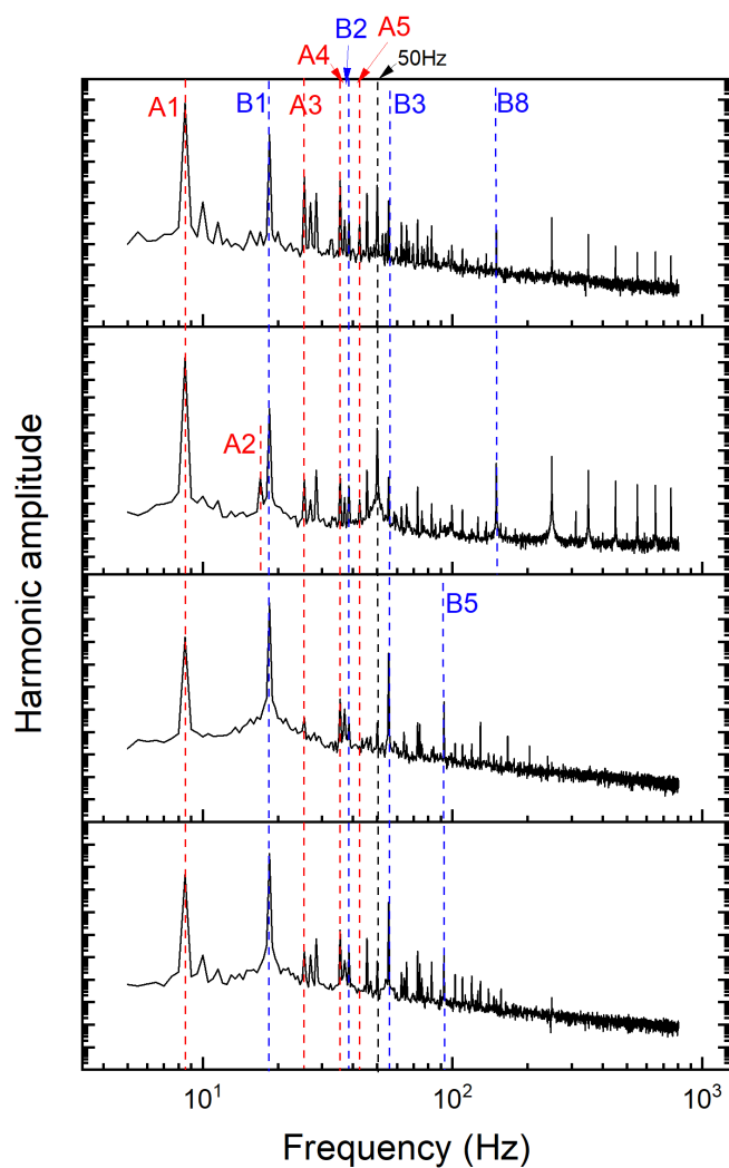
Figure S10. Two sinusoidal signals, signal A at 8.5 Hz and signal B at 18.5 Hz (peak-to-peak amplitude V_{PP} = 2 V for both) are applied at two electrodes of the POM-NMN. At the other 4 outputs, the currents are measured by a transimpedance amplifier and fed to the dynamic signal analyzer for FFT analysis. The HHG peaks are labeled as A_i ( i = 1 for the fundamental, i = n for the n^{\text{th}} harmonic, n is an integer) and B_i for harmonics corresponding to the A and B
