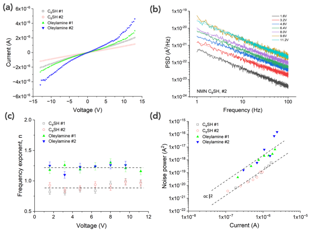
Figure 2. (a) Current-voltage (I-V) curves for the two PEs (labels #1 and #2) for the C_8SH -NMN and oleylamine-NMN. (b) Current power spectral density (PSD) S_i(f) , versus frequency for the C_8SH -NMN, PE #2 measured at several applied voltages (straight lines are the fits by a power law). (c) Frequency exponent, n , versus the applied voltage. (d) Noise power (NoP, i.e. the PSD, S_i(f) , integrated over the scanned frequency range 1-100 Hz) versus the DC current, which is taken from the
