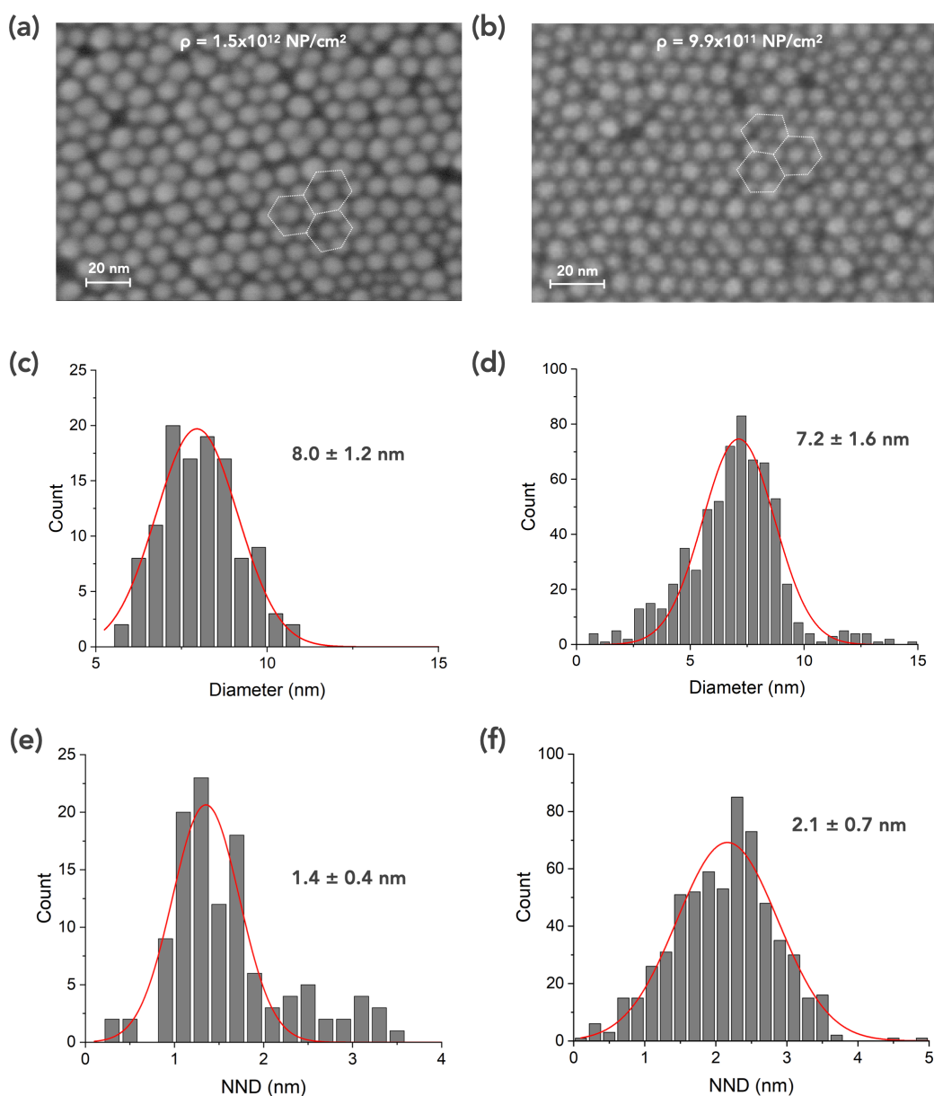
Figure S4. (a-b) Scanning electron microscope images of the PW 11 SH-NMN for batches 1 and 2 (magnification 652.75k and 162.96k, respectively). The hexagonal packing of the functionalized AuNP is illustrated by the dotted white lines in the panel. (c-d) Histograms of the AuNP diameter for the NMNs of batch 1 and batch 2, respectively. (e-f) Histograms of the nearest neighbor distance
