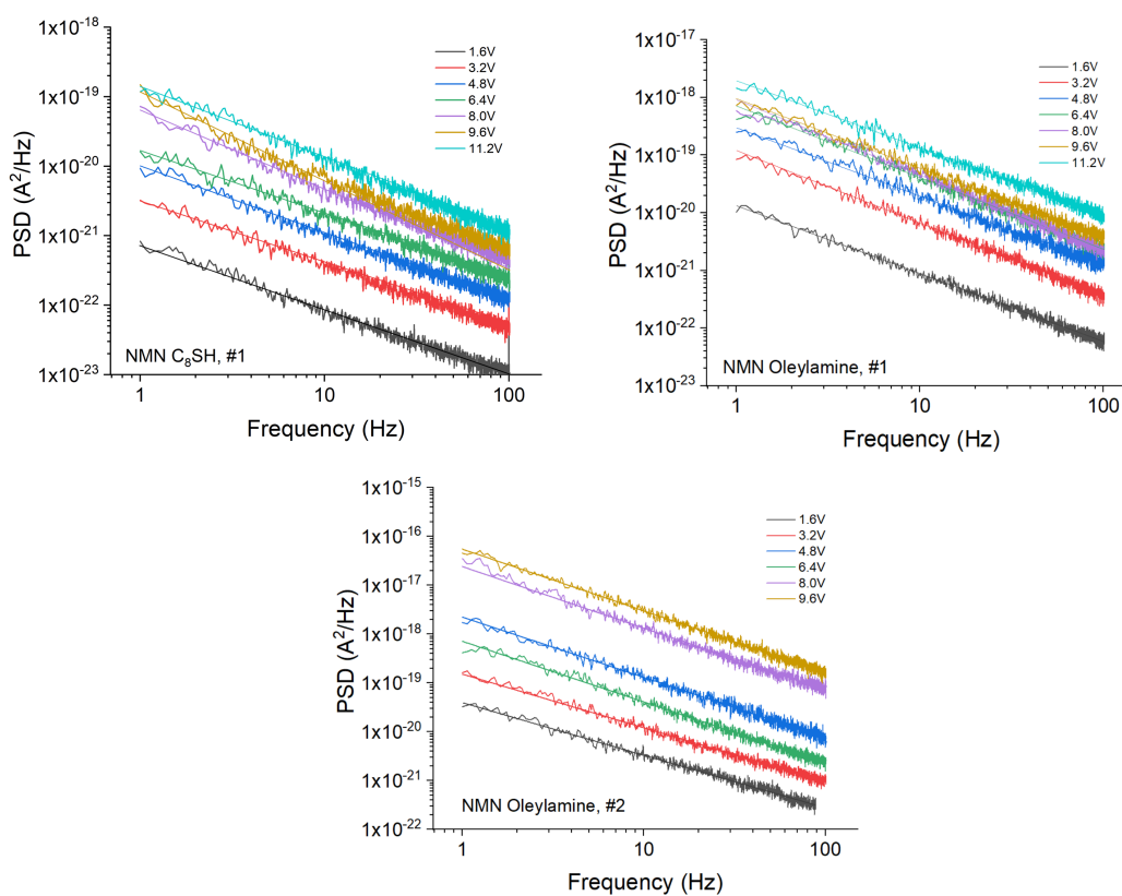
Figure S6. Current power spectral density (PSD), S_I(f) , versus frequency for the C 8 SH-NMN, PE #1, and the two PEs of the oleylamine-NMN, measured at several applied voltages.
