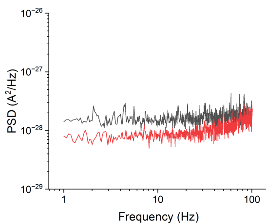
Figure S11. Noise floor of the setup measured for the two channels (the two trans-impedance amplifiers and the two-channel digital signal analyzer) with the prober tips raised (no sample).
