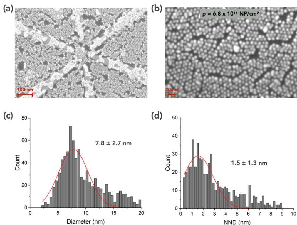
Figure S3. (a-b) Scanning electron microscope images of the C 8 SH-NMN at different magnifications (132.41k and 279.91k, respectively). The panel (a) shows the 6 electrodes and the monolayer of C 8 -AuNPs, the central ring between the
