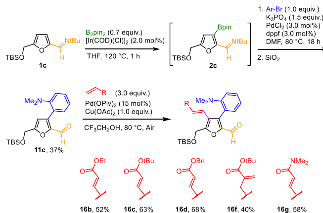
Scheme 8. Synthesis of peri-substituted furan derivatives.
