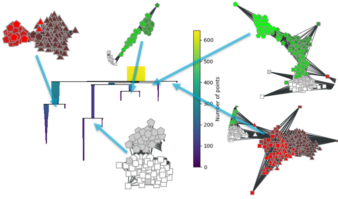
Fig. 8. Condensed clustering tree [3] obtained with our Hypergraph-Percol method on the \ell^2 -normalized olive oil dataset [8], [9]. We recover 8 of the 9 geographical ‘ground-truth’ region clusters. The resulting clustering is given in Tab. II.
