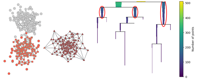
Fig. 7. Left: Results of our algorithm on the 3-blobs. Colours are the 3 ground-truth clusters: gray, orange and red. © Scikit-Learn’s Clustering webpage. Shapes are the final clustering using the condensed clustering tree [3] (Right). We recover the 3 clusters (triangles, squares and pentagons). Disks are unlabelled points.
