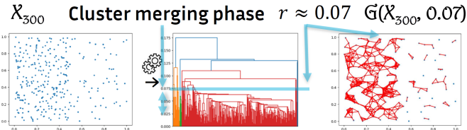
Fig. 3. From left to right: 1) The point cloud \mathcal{X}_{300} . 2) The dendrogram of the Single-Linkage applied on \mathcal{X}_{300} . 3) The geometric graph \mathcal{G}(\mathcal{X}_{300}, 0.07) .
