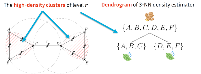
Fig. 4. Left: A cloud \mathcal{X}_6 of six points: two equilateral triangle at equidistance r . In red, the two clusters of H_{\hat{f}_{3\text{-NN}}} for level r . Right: The resulting dendrogram of the discrete hierarchical clustering H_{\hat{f}_{3\text{-NN}}} .
