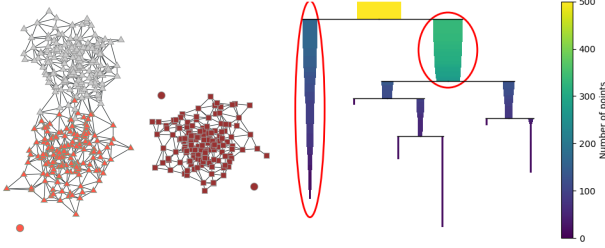
Fig. 5. Left: Result of HDBSCAN on the 3 blobs [7]. Colours are the 3 ground-truth clusters, Shapes are the clustering: only 2 clusters (triangles and squares). Disks are unclustered points. Right: The condensed clustering tree with the choice of clusters according to the excess of mass criterion [3].
