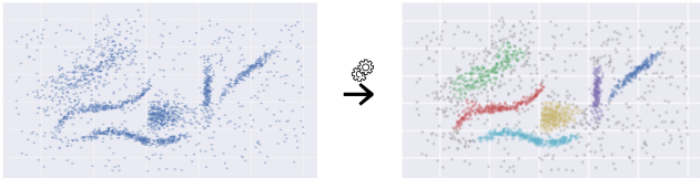
Fig. 1. Result of the Hierarchical Density-Based SCAN (HDBSCAN) algorithm [2] on a 2D toy dataset [3].
