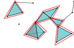
Fig. 6. A hypergraph and its five 2-Polyhedra (or ‘Triangle-connected’ components) surrounded in red.
