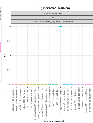
Figure 52: Human Stature data, k -RR Comb mechanism, max probability 0.1.
