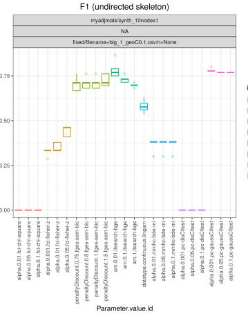
Figure 153: Synthetic 10 nodes data, Geometric mechanism, max probability 0.1.
