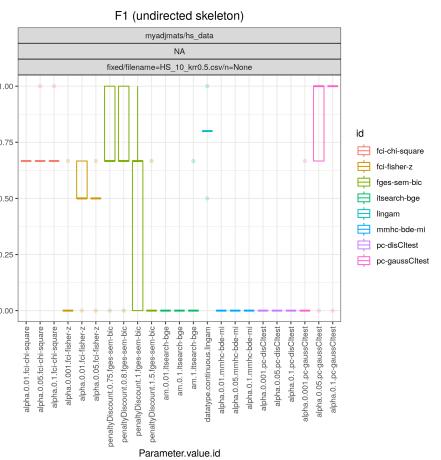
Figure 59: Human Stature data, k-RR C-wise mechanism, max probability 0.5.
