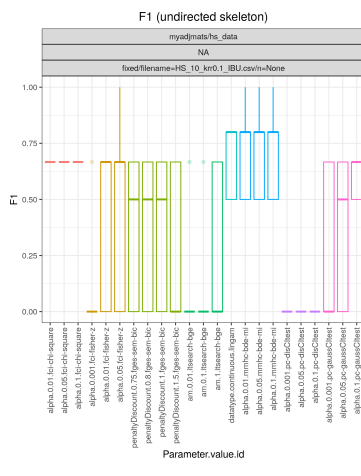
Figure 51: Human Stature data, k -RR C-wise IBU mechanism, max probability 0.1.
