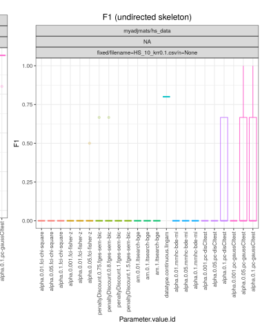
Figure 50: Human Stature data, k -RR C-wise mechanism, max probability 0.1.
