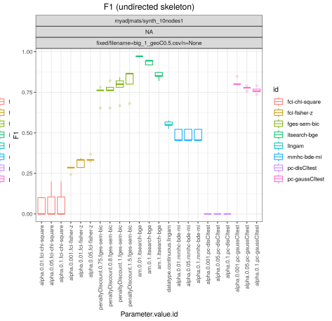
Figure 158: Synthetic 10 nodes data, Geometric mechanism, max probability 0.5.
