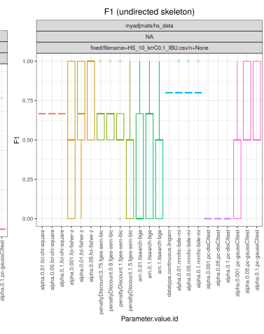
Figure 53: Human Stature data, k -RR Comb IBU mechanism, max probability 0.1.
