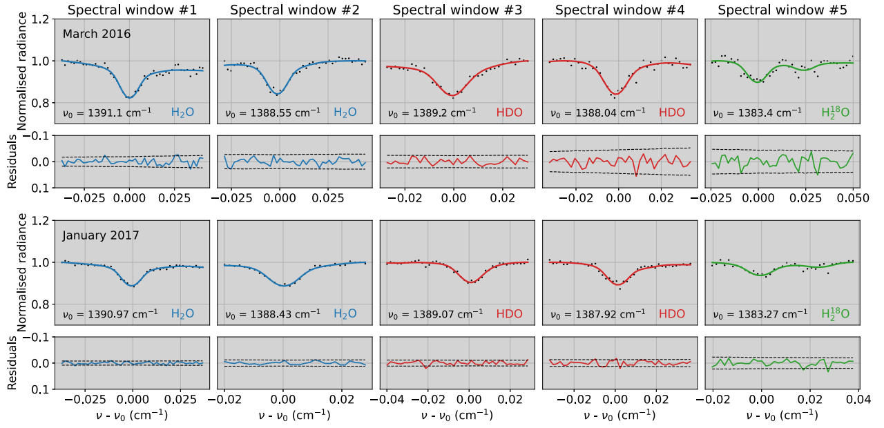
Figure 5. Example of spectral fits to the SOFIA/EXES data. The different rows of panels represent examples of the spectral fits in the observations made in 2016 March and 2017 January. The different columns represent the spectral fits for each of the spectral windows selected to derive the abundance of the different water isotopes. In the upper panels of each row, the dots are the SOFIA/EXES measurements, while the coloured lines represent the best fit to the data, with the colours representing the isotopologue the absorption lines correspond to. Finally, the lower panels show the residuals between the best fit and the data (coloured lines), while the dashed lines represent the uncertainties of the measurement.
