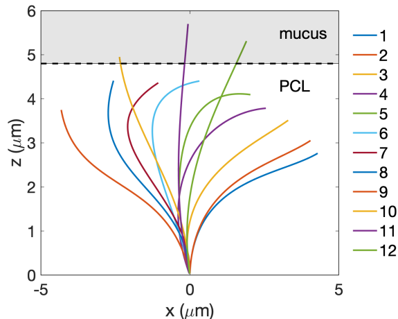
FIGURE 1. Traces of a cilium during one period of its beat with a PCL-mucus interface at z = 4.8 \mu\text{m} . Description made by Sanderson and Sleigh [42, 43].
