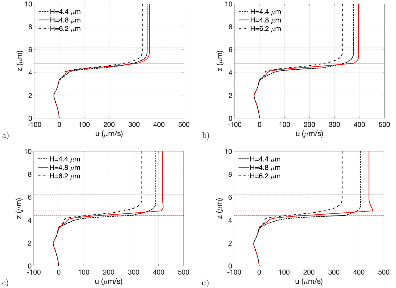
FIGURE 11. Influence of the position of the ASL ( H ) on the mean axial velocity z \mapsto \overline{u_x^{x,y}}(z) in the radial direction (through PCL and mucus). a) \mu_2 = 2 \times 10^0 mPa·s, b) \mu_2 = 5 \times 10^0 mPa·s, c) \mu_2 = 1 \times 10^1 mPa·s, d) \mu_2 = 1 \times 10^4 mPa·s.
