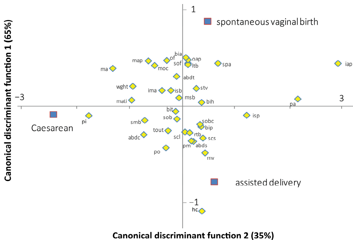
Figure 3. Standardized canonical coefficients of the fetal-pelvic variables between the two canonical discriminant functions, based on modern human data. mati: maximal transverse diameter of the inlet; pi: posterior inlet diameter; pa: pectineal angle; isb: inlet sacral breadth; iap: inlet antero-posterior diameter; map: midplane antero-posterior diameter; isp: interspinous diameter; msb: midplane sacral breadth; pm: posterior midplane diameter; ma: midplane angle; tout: transverse outlet diameter; spa: subpubic angle; po: posterior outlet diameter; oap: outlet antero-posterior diameter; ima: inlet–midplane angle; scl: sacral chord length; scs: sacral chord subtense; smb: submentobregmatic diameter; sob: suboccipitobregmatic diameter; sof: suboccipitofrontal diameter; mv: mentovertical diameter; moc: mento-occipital diameter; of: occipitofrontal diameter; bip: biparietal diameter; bit: bitemporal diameter; rtb: right trasion–bregma diameter; ltb: left trasion–bregma diameter; sobc: suboccipitobregmatic circumference; bia: biacromial diameter; stv: sternum–thoracic vertebral diameter; abdc: abdominal circumference; abds: abdominal sagittal diameter; abdt: transverse abdominal diameter; bih: bitrochanterian diameter; wght: birthweight.
