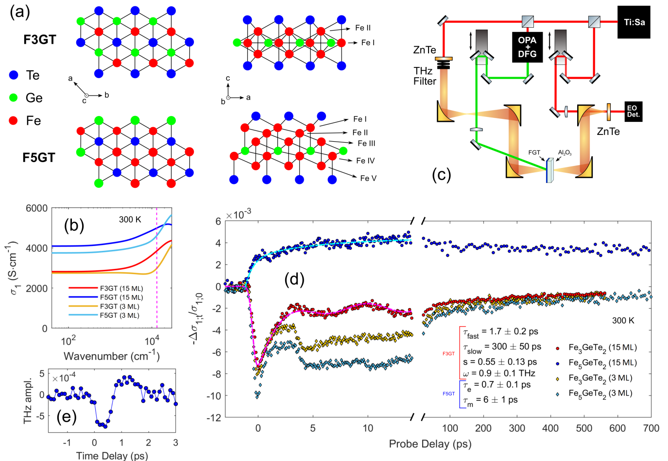
FIG. 1: | Crystal structure and Optical pump-THz probe measurements of \text{Fe}_n\text{GeTe}_2 ( n = 3, 5 ) films. a) Crystal structure as seen from two different points of view for \text{Fe}_3\text{GeTe}_2 (F3GT) and \text{Fe}_5\text{GeTe}_2 (F5GT). For simplicity, the Fe I atoms are represented only near the Te top plane. In reality, they are distributed near both Te layers, forming two partially occupied sub-lattices 15,27 . b) Real part of optical conductivity for the four measured films, as extracted through a multi-layer stacking model. The pink dotted line identifies the 800 nm ( 12500 \text{ cm}^{-1} ) pump wavelength. c) Optical pump-THz probe spectroscopy setup. An initial seed laser (800 nm, 30 fs, 7 mJ) is split twice to create a probe THz signal through optical rectification in a ZnTe crystal (0.5 mm), a pump signal at variable wavelength through an optical parametric amplifier and difference frequency generation (OPA+DFG) system, and a final optical signal to probe the THz electric field through an electro-optical (EO) detection in a second ZnTe crystal (0.3 mm). d) Pump-probe data at 300 K and 5 \text{ mJ/cm}^2 for the four measured films over an extended time scale. The discontinuous curves overlaid to the experimental data represent the best fits according to Eq. 1 and a bi-exponential type-II demagnetization, respectively for the 15 ML F3GT and F5GT films. The best-fit parameters are indicated in the inset. e) Light-induced demagnetization THz emission from a 15 ML F5GT film.
