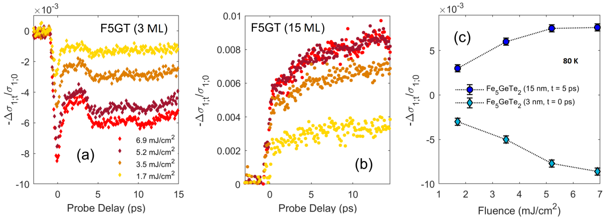
FIG. 3: | Optical pump-THz probe fluence dependent measurements of \text{Fe}_5\text{GeTe}_2 films. a-b) Fluence dependence of the 80 K pump-probe trace for F5GT films of 3 and 15 ML, respectively. c) Fluence evolution of the pump-probe trace at fixed probe delays for the 3 and 15 ML films of F5GT at 80 K.
