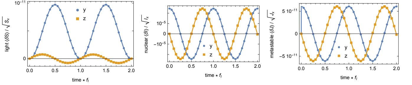
Figure 6: Comparison between the full model Eq. (71) and the same model after adiabatic elimination of the F = 1/2 and tensor degrees of freedom in “Config.2”. The nuclear magnetization is set to M = 98\% . Blue indicates the y spin component, while yellow the z spin component. Solid lines are the full model, while round and square markers indicate the numerical solution of the same model after adiabatic elimination of the F = 1/2 and tensor degrees of freedom (without setting \mu = \chi = 0 , as done in Fig. (4)). Simulation parameters: n_{\text{ph}}/N_{\text{cell}} = 10^{-3} , N_{\text{cell}}/n_{\text{cell}} = T/\tau = 10^6 s, and an initial state resulting from tilting the nuclear spin by 0.01 rad. Time is in units of the nuclear spin Larmor frequency.
