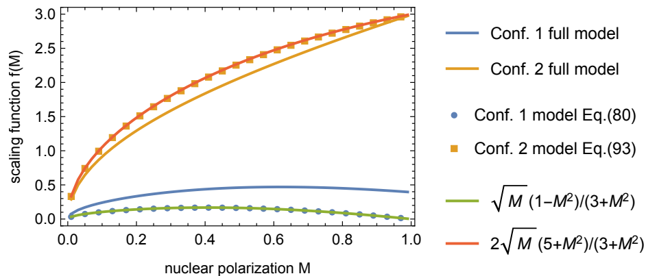
Figure 5: Comparison between the effective light-nuclear spin coupling factor in “Config.1” and “Config.2” as a function of the nuclear spin magnetization M . Blue indicates “Config.1”, while yellow “Config.2”. Solid lines refer to the coupling extracted from the full model, while round and square markers refer to the coupling extracted from Eq. (80) and Eq. (93), respectively. Red and green lines are the analytical expressions obtained for B_x = 0 , namely Eq. (91) and Eq. (104) respectively. Simulation parameters: n_{\text{ph}}/N_{\text{cell}} = 10^{-3} and N_{\text{cell}}/n_{\text{cell}} = T/\tau = 10^6 s.
