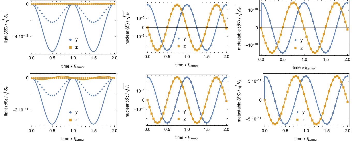
Figure 3: Comparison between the full model Eq. (71) and the simplified model Eq. (80) in “Config.1”. Top row is for a nuclear magnetization of M = 2\% , while the bottom row is for M = 10\% . Blue indicates the y spin component, while yellow the z spin component. Solid lines are the full model, while round and square markers indicate the numerical solution of Eq. (80). Simulation parameters: n_{\text{ph}}/N_{\text{cell}} = 10^{-3} , N_{\text{cell}}/n_{\text{cell}} = T/\tau = 10^6 s, and an initial state resulting from tilting the nuclear spin by 0.01 rad. Time is in units of the nuclear spin Larmor frequency.
