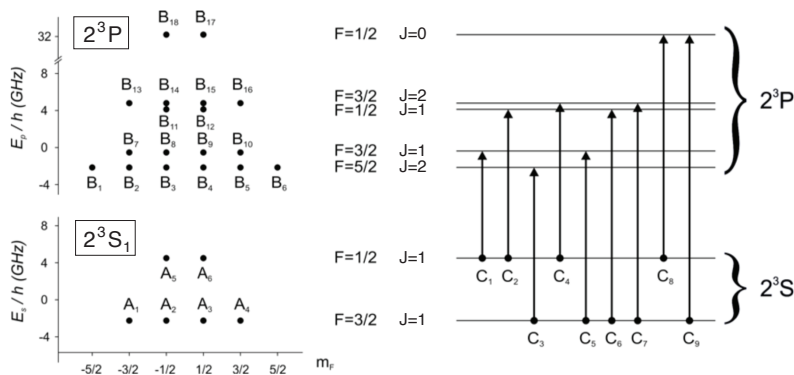
Figure 1: Left: hyperfine structure of states 2^3S_1 and 2^3P in ^3\text{He} . Right: allowed transitions at 1083 nm.
