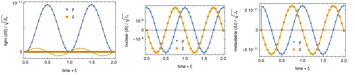
Figure 4: Comparison between the full model Eq. (71) and the simplified model Eq. (93) in “Config.2”. The nuclear magnetization is set to M = 98\% . Blue indicates the y spin component, while yellow the z spin component. Solid lines are the full model, while round and square markers indicate the numerical solution of Eq. (93). Simulation parameters: n_{ph}/N_{cell} = 10^{-3} , N_{cell}/n_{cell} = T/\tau = 10^6 s, and an initial state resulting from tilting the nuclear spin by 0.01 rad. Time is in units of the nuclear spin Larmor frequency.
