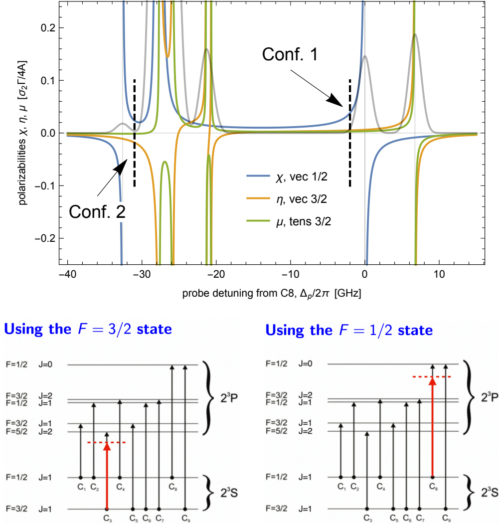
Figure 2: Top: Coupling constants \chi Eq. (8) (blue line), \eta Eq. (9) (orange line) and \mu Eq. (10) (green line) for the F = 1/2 and F = 3/2 levels of the ^3\text{He} metastable, as a function of the light frequency detuning \Delta_p taking the C_8 transition as the origin. All the constants are divided by the constant 4A/(\sigma_2\Gamma) . The grey line shows the absorption spectrum taking into account the Doppler broadening for T = 300 K for a non polarized sample [14]. Two possible operating point marked as “Config.2” at \Delta_p/(2\pi) = -31 GHz and “Config.1” at \Delta_p/(2\pi) = -2 GHz are discussed in the text. Bottom: Level scheme depicting the two possible operating point marked as “Config.2” and “Config.1”, respectively.
