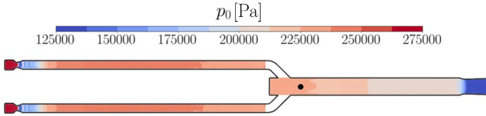
Fig. 3: Mean pressure field p_0 in the median plane along the z-axis. The black dot is the location of the pressure sensor mentioned in 2.2.
