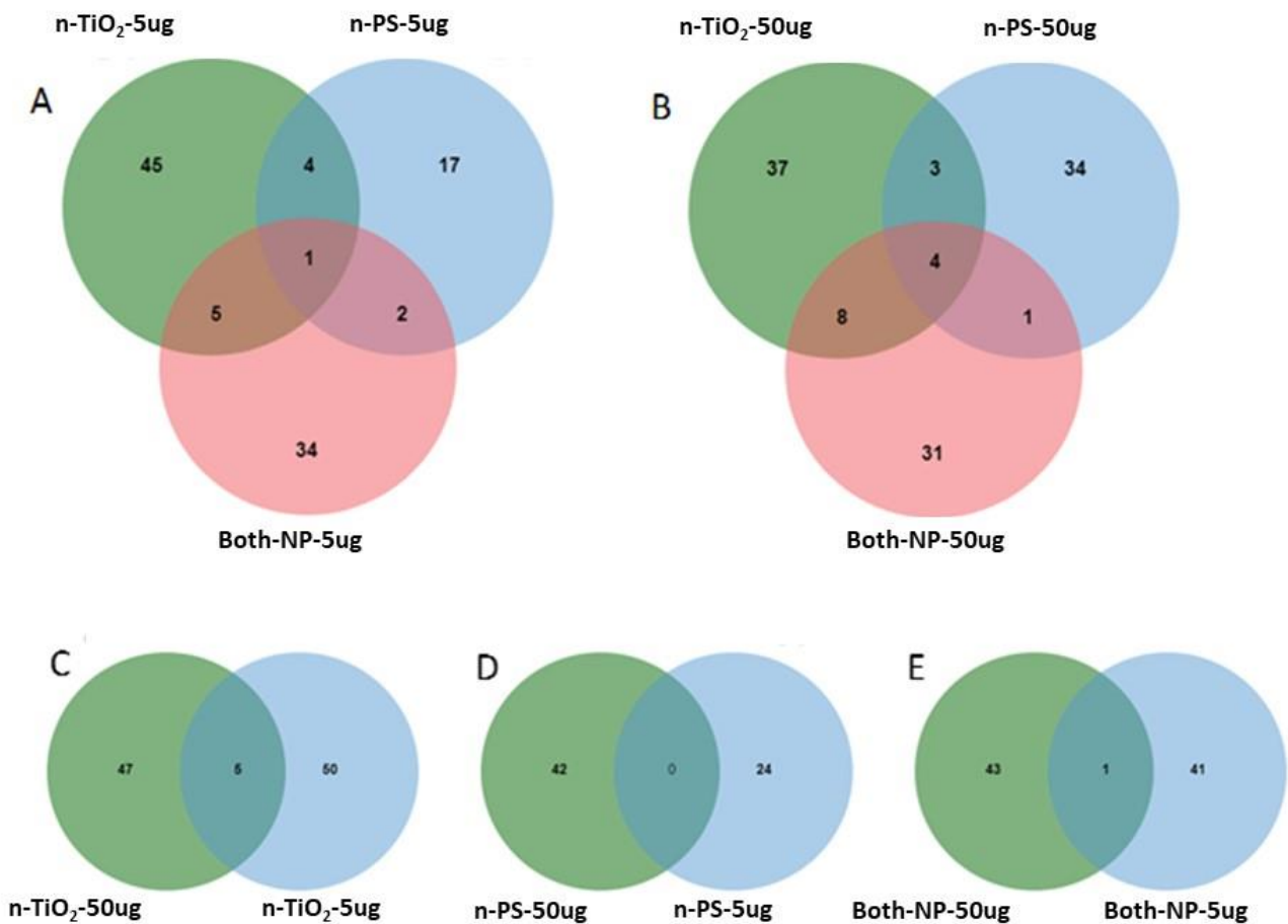
Fig. 4. Venn diagrams showing shared Differentially Expressed Genes (DEG) when comparing individuals exposed to control end experimental conditions at 5 \mu\text{g/L} (A) and 50 \mu\text{g/L} (B). The green circles represent the n-TiO 2 conditions, the blue ones the PS-COOH NP conditions and the pink ones the co-exposure to both nanoparticles. The overlaps of circles represent the shared DEG. Barplots show DEG numbers by conditions with the same colors of circles. Venn diagrams showing shared transcripts between pair of conditions for n-TiO 2 (A), PS-COOH NP (B) and combined exposure (C). Green circles represent the 50 \mu\text{g/L} treatments for each pollutant and the blue ones represent the 5 \mu\text{g/L} treatments. The overlaps of the circles represent the shared transcripts.
