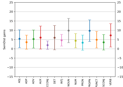
Fig. 5: SemDist gains for each POS tag corrected.
