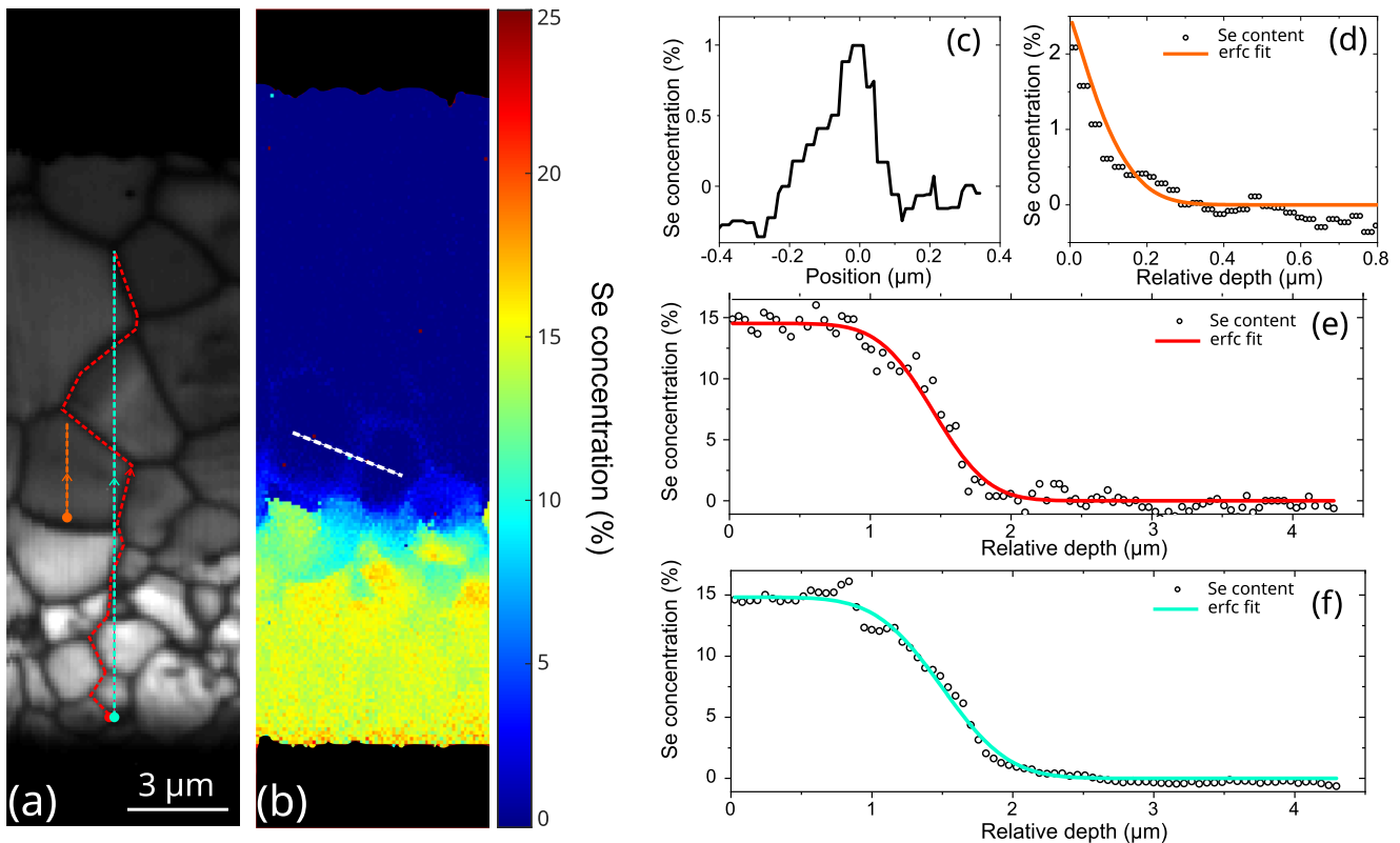
FIG. 4. (a) RT panchromatic map of CdSe 0.2 Te 0.8 , where the analyzed line profiles are indicated by the colored dotted lines. (b) Corresponding Se concentration map emphasizing a higher Se content in GB. (c) Se concentration profile across one of the grain boundaries [white dotted line in (b)]. (d)–(f) Data and fits of selenium concentration in-depth profiles. The color of the fit matches the indicated lines in (a). The colored dots and the arrows in panel (a) indicate the origin and the positive direction along the linescan, respectively. The relative depth in (d)–(f) corresponds to the vertical position of pixels in the layer.
