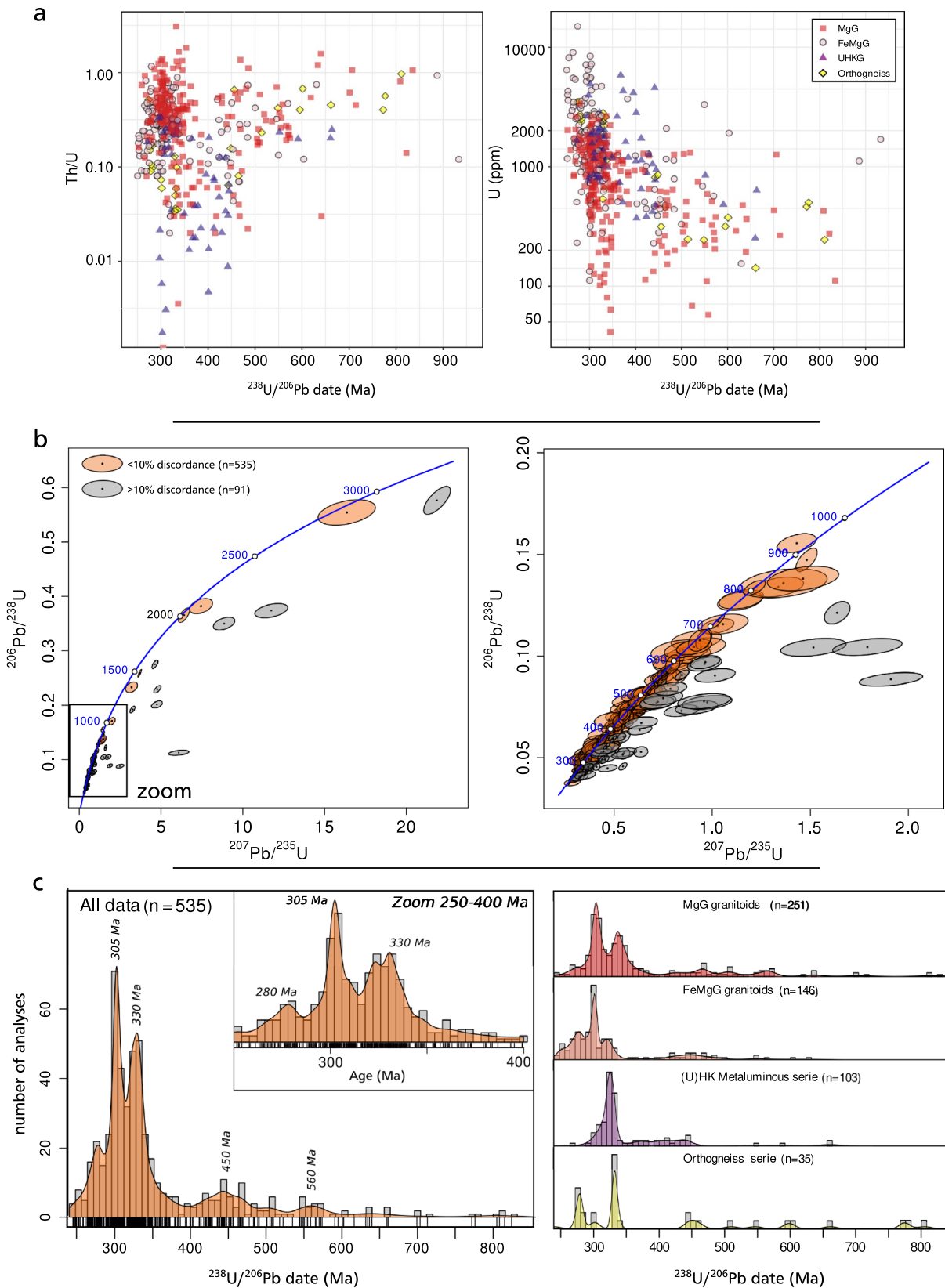
Fig. 9 Summary of U–Pb data. a Th/U and U content of dated zircon spots versus ^{238}\text{U}/^{206}\text{Pb} dates. b Zircon U–Pb concordia diagrams of all data, and zoomed on dates < 1000 Ma. c Histograms and Kernel Density Estimates (KDE) of ^{238}\text{U}/^{206}\text{Pb} dates, for the full dataset and splitted by magmatic series
