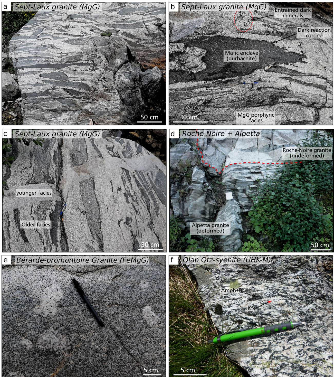
Fig. 4 Field photos of the different magmatic facies. a Swarm of elongated durbachitic (mafic ultrapotassic. UHKM) enclaves in a boulder of the Sept-Laux granite (MgG). b Close-up view of one enclave, showing digitated borders with a reaction rim enriched in mafic minerals (Bt, Amp). Clusters of dark minerals in the granite could represent xenocrysts from the mafic enclaves entrained into the melt. c, d Contact between older and younger intrusions in the Sept-Laux granite and at the contact between Alpetta (older) and
