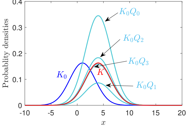
FIGURE 1. Demonstration of the convergence of the expansion for a Gaussian process. We plot the short-time propagator K_0 , the full propagator K , and low-order approximations K_0 Q_0 , K_0 Q_1 , K_0 Q_2 , and K_0 Q_3 , to show the convergence K_0 Q_m \rightarrow K when m \rightarrow \infty . We adopted the parameter values H_0 = -1 , G_0 = 1 , y = 1 , t_0 = 0 , t = 3 (in arbitrary units).
