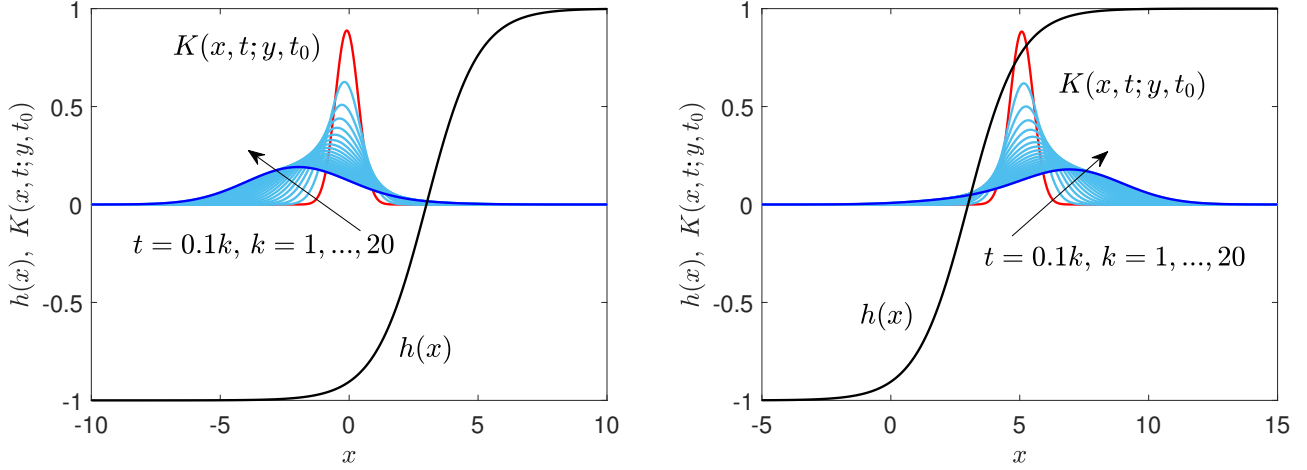
FIGURE 8. Stochastic process with a sigmoidal drift. We plot the full propagators K given in Eq.(141) for different values of the time t = 0.1k , with k = 1, \dots, 20 (start time in red and end time in blue). We also plot the sigmoidal drift h(x) (black lines). We adopted the parameter values, G_0 = 1, H_0 = 1, t_0 = 0, S = 10 , and \alpha = 1/2 (in arbitrary units). We observe a regressive diffusion in left panel with y = 0 , and a progressive diffusion in the right panel with y = 5 .
