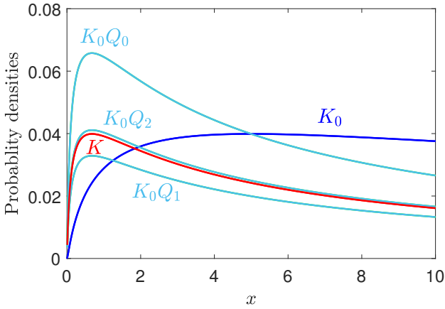
FIGURE 2. Convergence of the short-time expansion for a geometric Brownian process. We plot the short-time propagator K_0 , the full propagator K , and some low-order approximations K_0 Q_0 , K_0 Q_1 , and K_0 Q_2 , to illustrate the convergence K_0 Q_m \rightarrow K when m \rightarrow \infty . We adopted the parameter values H_0 = -1 , G_0 = 1 , y = 5 , t_0 = 0 , t = 2 , and \alpha = 1/2 (in arbitrary units).
