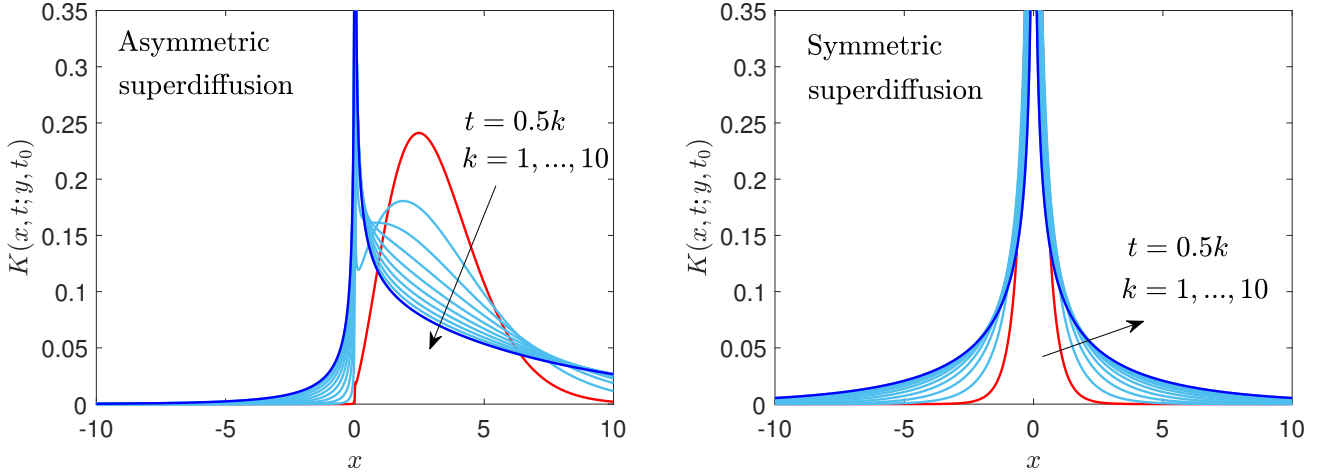
FIGURE 6. Asymmetric and symmetric superdiffusion processes. We plot the full propagators K given in Eqs.(114) and (115) for different values of the time t = 0.5k (start time in red and end time in blue), with k = 1, \dots, 10 , and for \beta = +1/2 ( e = 2 ). We adopted the parameters, G_0 = 1 , y = 3 (for the asymmetric superdiffusion, left panel), y = 0 (for the symmetric superdiffusion, right panel), t_0 = 0 , and \alpha = 1/2 (in arbitrary units).
