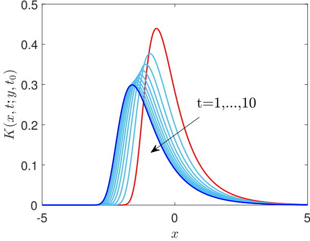
FIGURE 7. Example of time evolution for an exponential process. We plot the full propagator K given in Eq. (116) for different values of the time t = 1, \dots, 10 (start time in red and end time in blue). We adopted the parameter values G_0 = 1 , \gamma = 1 , y = 0 , t_0 = 0 , and \alpha = 1/2 (in arbitrary units).
