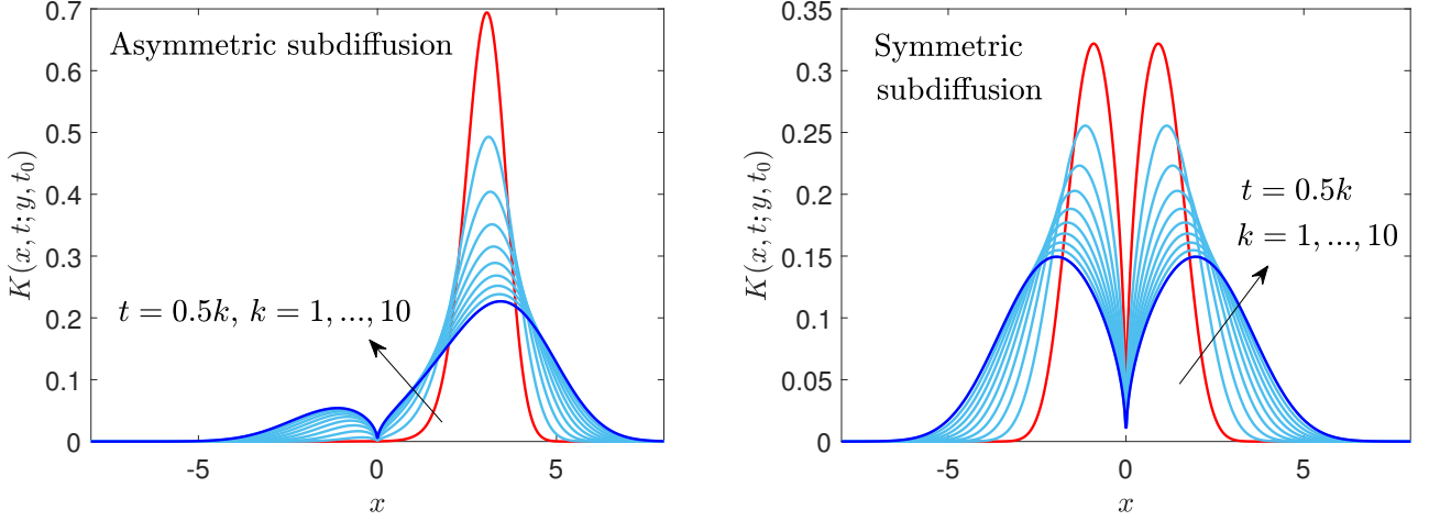
FIGURE 5. Asymmetric and symmetric subdiffusion processes. We plot the full propagators K given in Eqs.(114) and (115) for different values of the time t = 0.5k , with k = 1, \dots, 10 (start time in red and end time in blue), and for \beta = -1/2 ( e = 2/3 ). We adopted the parameters, G_0 = 1 , y = 3 (for the asymmetric subdiffusion, left panel), y = 0 (for the symmetric subdiffusion, right panel), t_0 = 0 , and \alpha = 1/2 (in arbitrary units).
