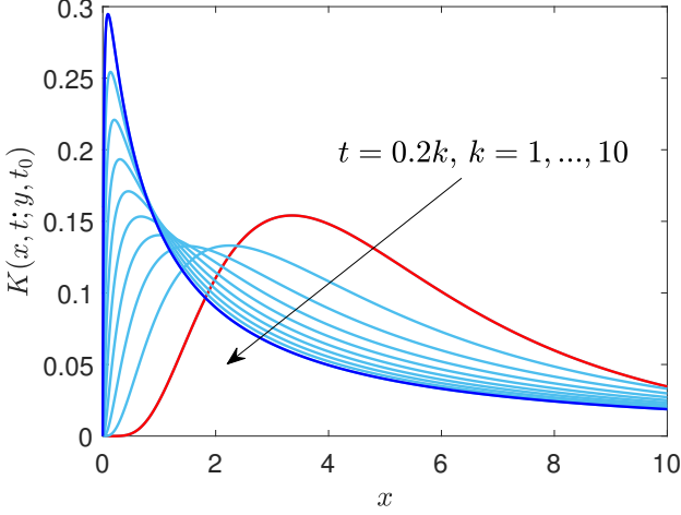
FIGURE 4. Example of time evolution for a geometric Brownian process. We plot the full propagator K given in Eq. (111) for different values of the time t = 0.2k , with k = 1, \dots, 10 (start time in red and end time in blue). We adopted the parameters, G_0 = 1 , y = 5 , t_0 = 0 , and \alpha = 1/2 (in arbitrary units).
