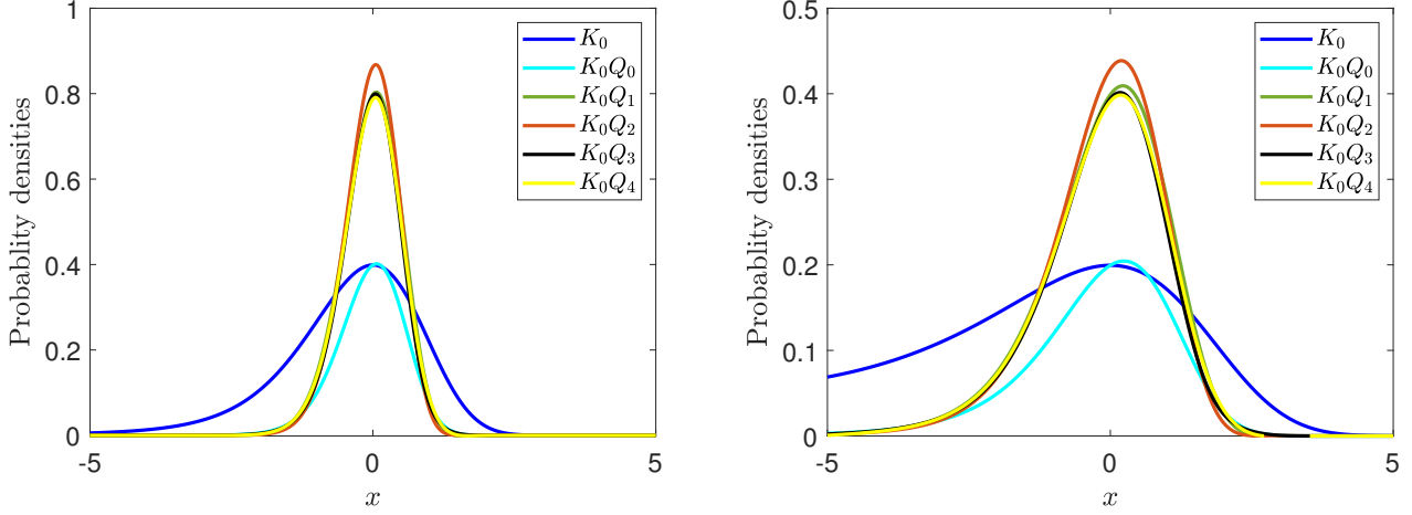
FIGURE 3. Application of the recursive procedure to the stochastic equation for the remodeler-nucleosome complex. In the left panel we adopted the parameters k = 2 , \beta = 1 , \gamma = 1/10 , and A = 1 , and in the right panel k = 2 , \beta = 1 , \gamma = 1/10 , and A = 2 (in arbitrary units). In both cases we plot the short-time propagator K_0 , and low-order approximations K_0Q_0 , K_0Q_1 , K_0Q_2 , K_0Q_3 , and K_0Q_4 , to show the convergence of K_0Q_m for m \rightarrow \infty . Here, Q_m = \sum_{n=0}^m F_n(x; y)(t - t_0)^n represents the partial sum of Eq. (31). In both panels we adopted t_0 = 0 , and t = 1/2 .
