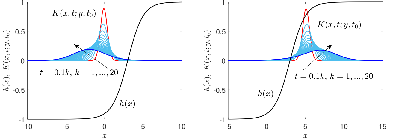
FIGURE 8. Stochastic process with a sigmoidal drift. We plot the full propagators K given in Eq.(141) for different values of the time t = 0.1k , with k = 1, \dots, 20 (start time in red and end time in blue). We also plot the sigmoidal drift h(x) (black lines). We adopted the parameter values, G_0 = 1, H_0 = 1, t_0 = 0, S = 10 , and \alpha = 1/2 (in arbitrary units). We observe a regressive diffusion in left panel with y = 0 , and a progressive diffusion in the right panel with y = 5 .
