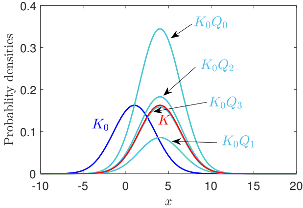
FIGURE 1. Demonstration of the convergence of the expansion for a Gaussian process. We plot the short-time propagator K_0 , the full propagator K , and low-order approximations K_0 Q_0 , K_0 Q_1 , K_0 Q_2 , and K_0 Q_3 , to show the convergence K_0 Q_m \rightarrow K when m \rightarrow \infty . We adopted the parameter values H_0 = -1 , G_0 = 1 , y = 1 , t_0 = 0 , t = 3 (in arbitrary units).
